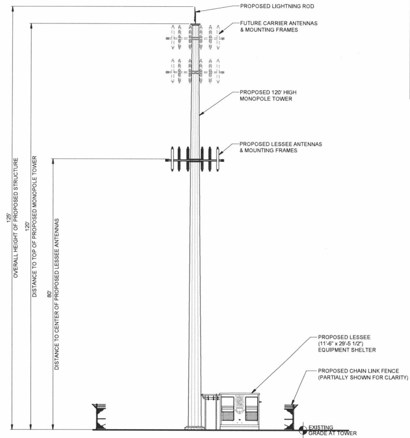
1 WEST ELEVATION
