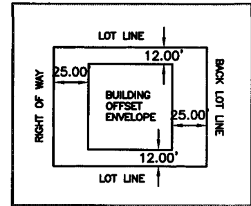
TYPICAL LOT DIMENSION
