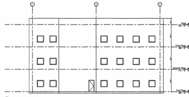
C4 WEST ELEVATION
