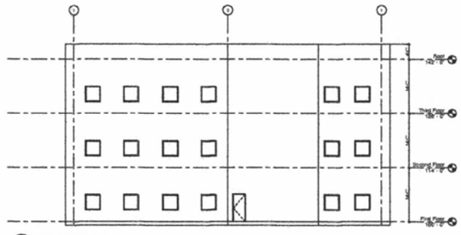
C1 EAST ELEVATION
