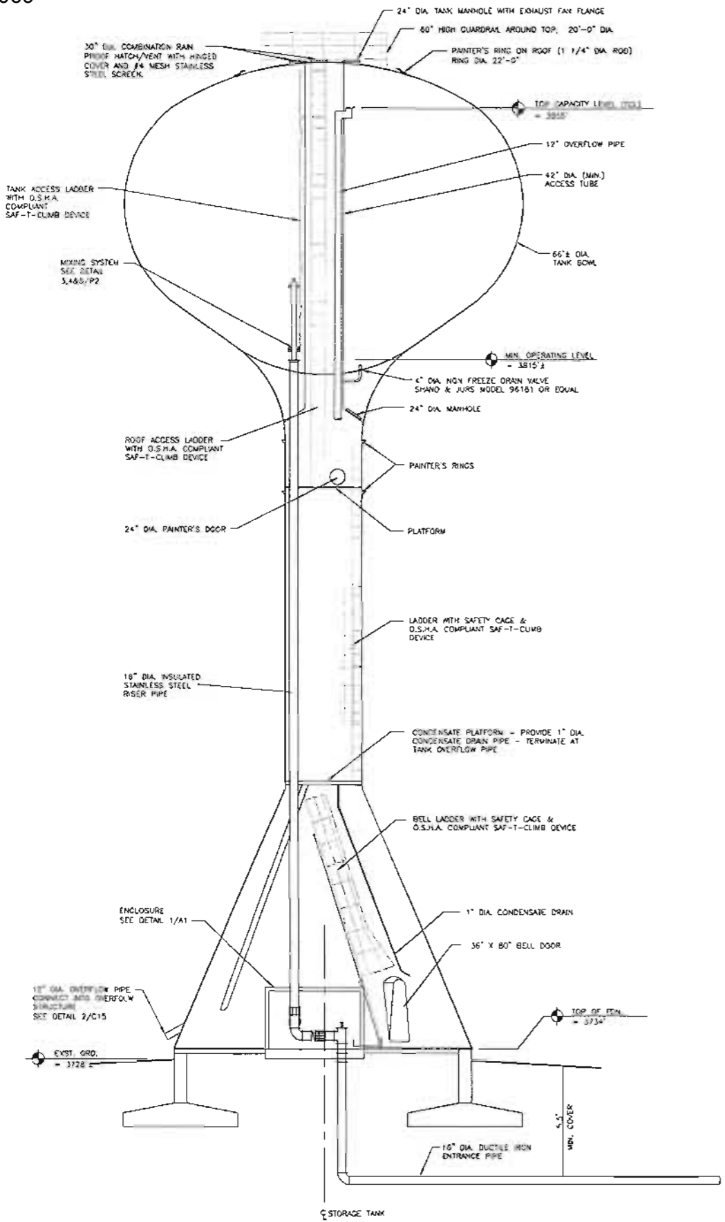
1 750,000 GALLON ELEVATED PEDESTAL SPHEROID STORAGE TANK SCALE: NONE
