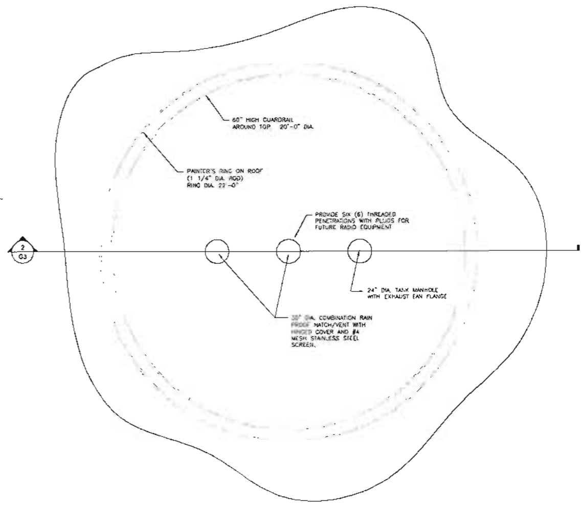
TOWER ROOF PLAN SCALE: NONE
