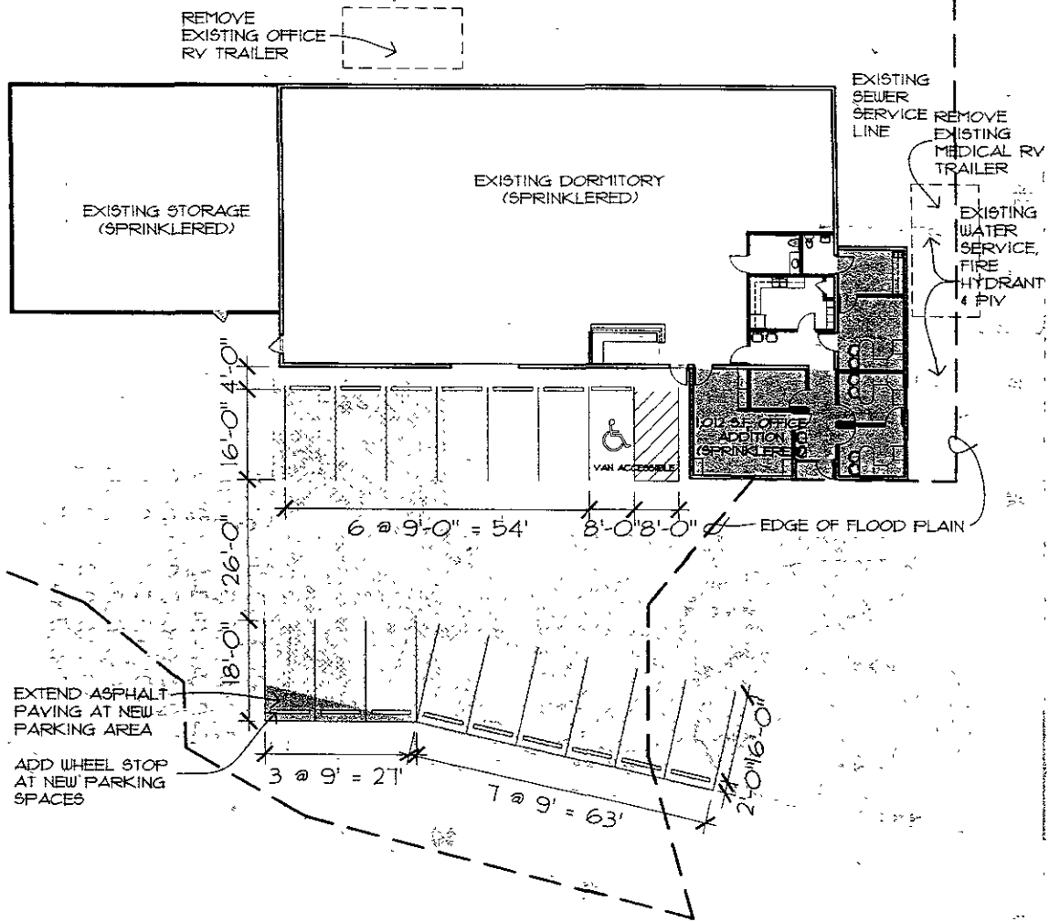
1 SITE PLAN ALL 1"=20'-0" NORTH
