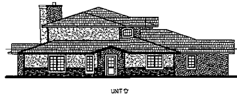
WEST ELEVATION
