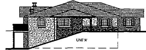
EAST ELEVATION
