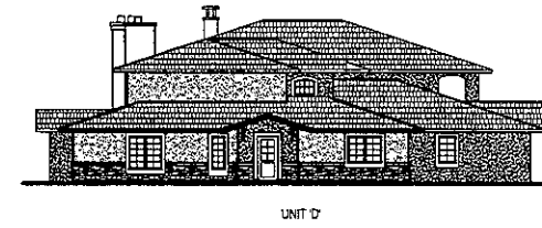
WEST ELEVATION
