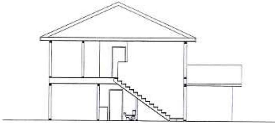
1 SECTION A3.1 1/8"=1'-0"
