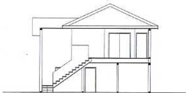
1 SECTION B3.1 1/8"=1'-0"
