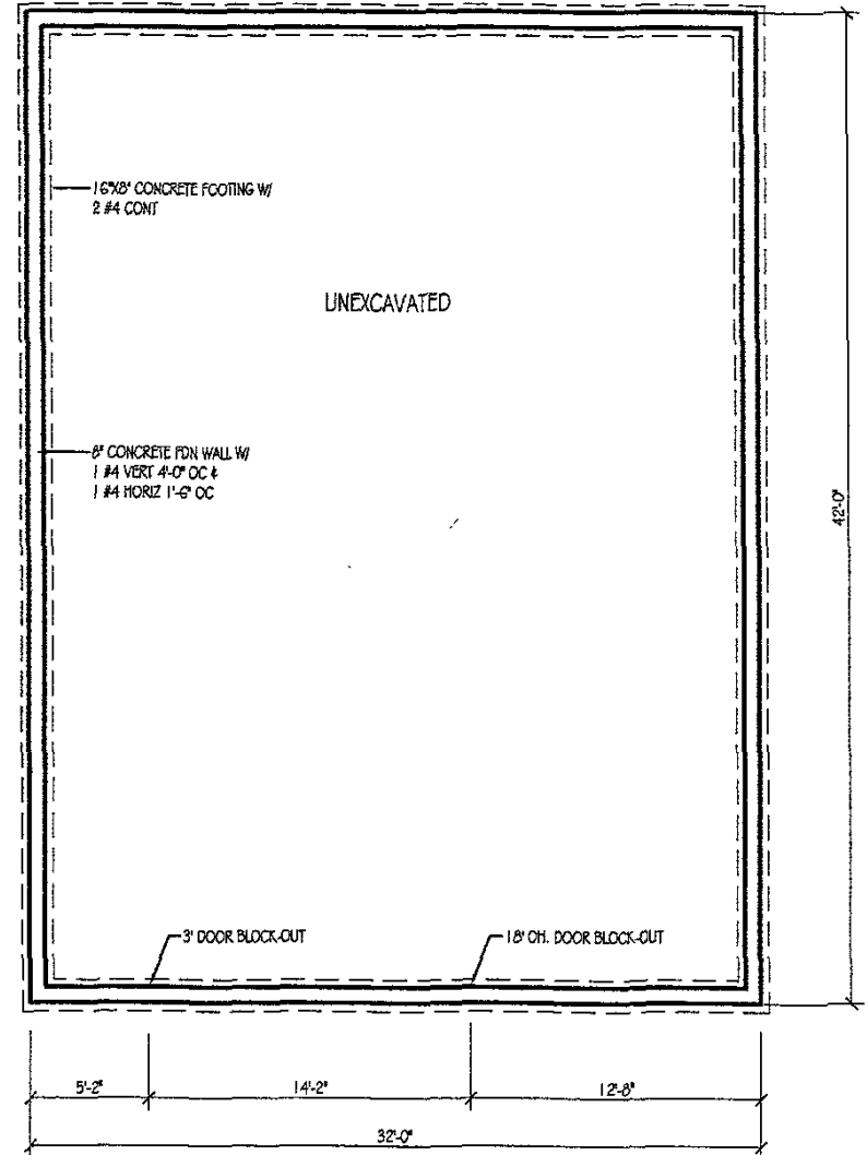
FOUNDATION PLAN
