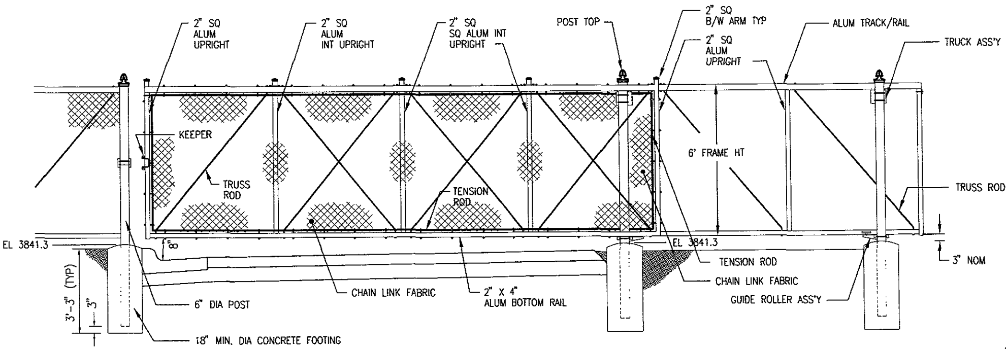
CHAIN LINK MANUALLY OPERATED SLIDING GATE DETAIL
