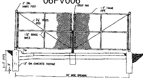
CHAIN LINK GATE DETAIL
