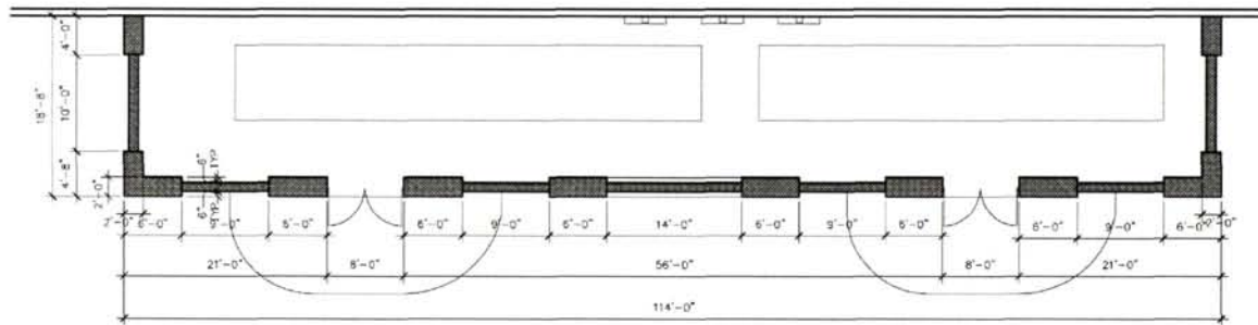
1 COMPRESSOR HOUSE FLOOR PLAN
