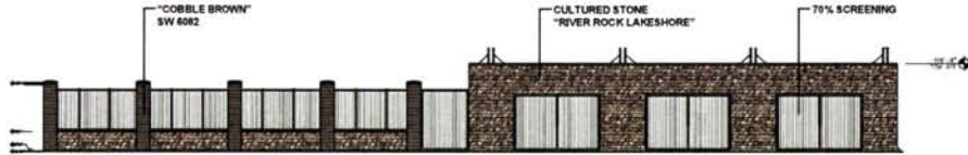
2 GARDEN CENTER ELEVATION
