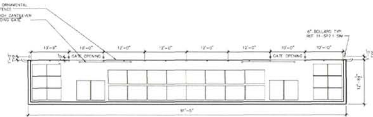
1 BALE AND PALLET RECYCLING AREA SCREENING PLAN—ORNAMENTAL GATES
