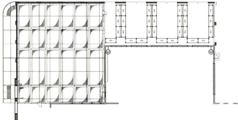
1 GARDEN CENTER FLOOR PLAN
