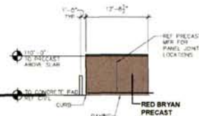
3 SIDE ELEVATION
