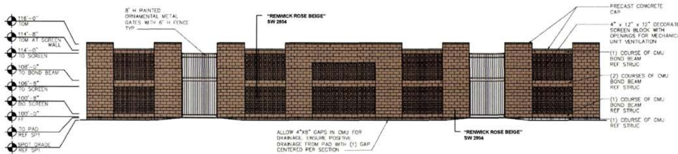
2 COMPRESSOR HOUSE ELEVATION
