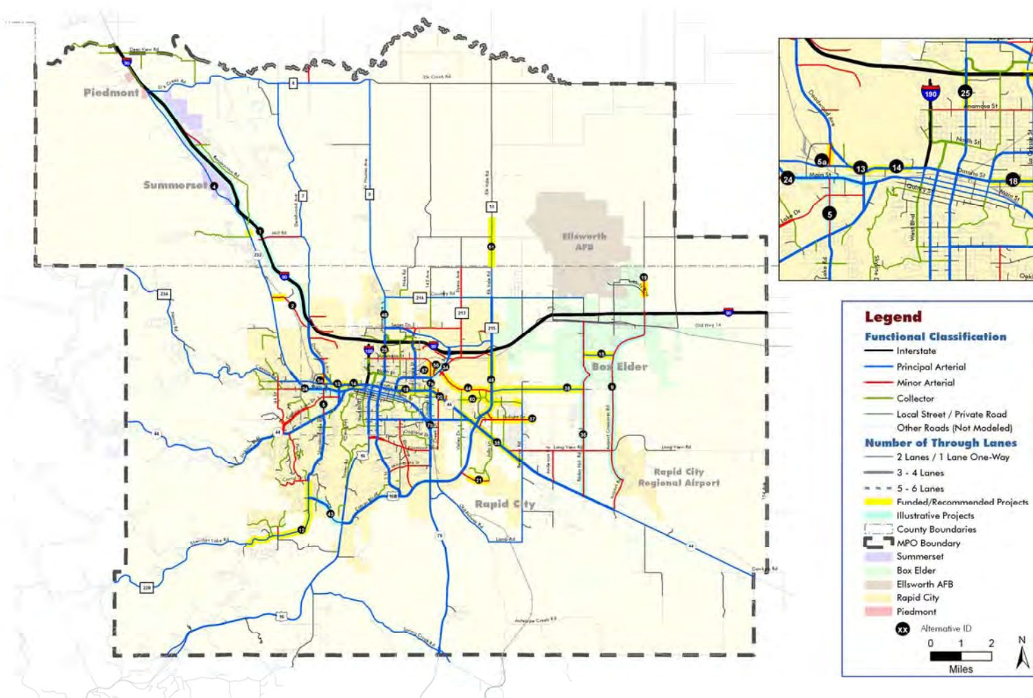
Figure 7-6: Recommended Financially Constrained Roadway Plan
