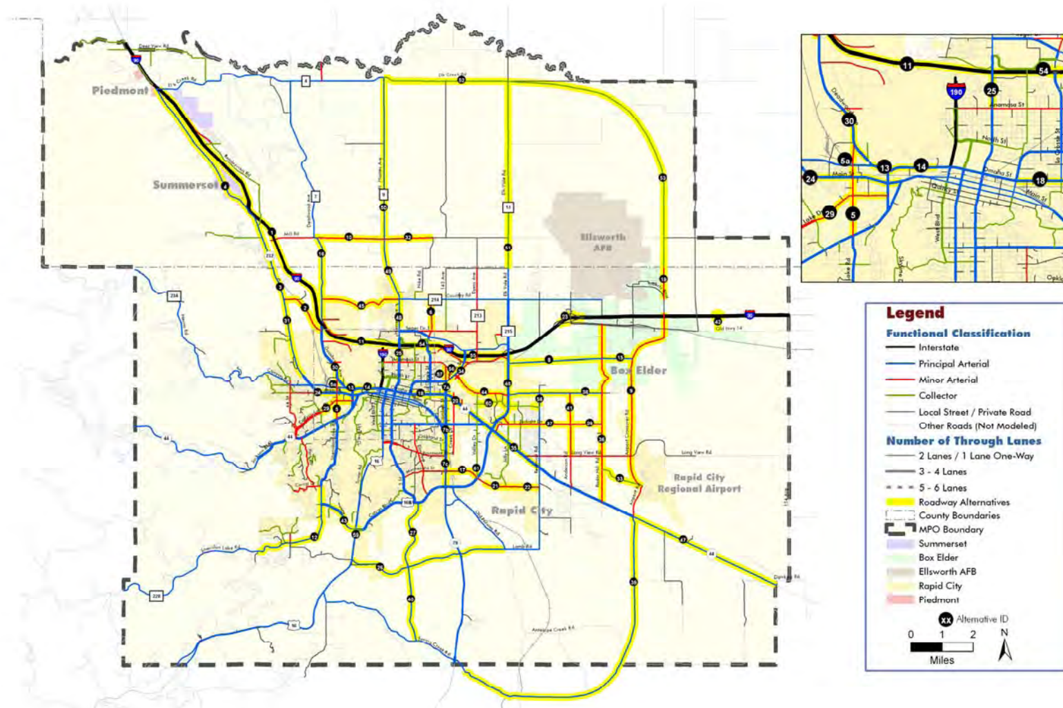
Figure 7-5: Roadway Alternatives
