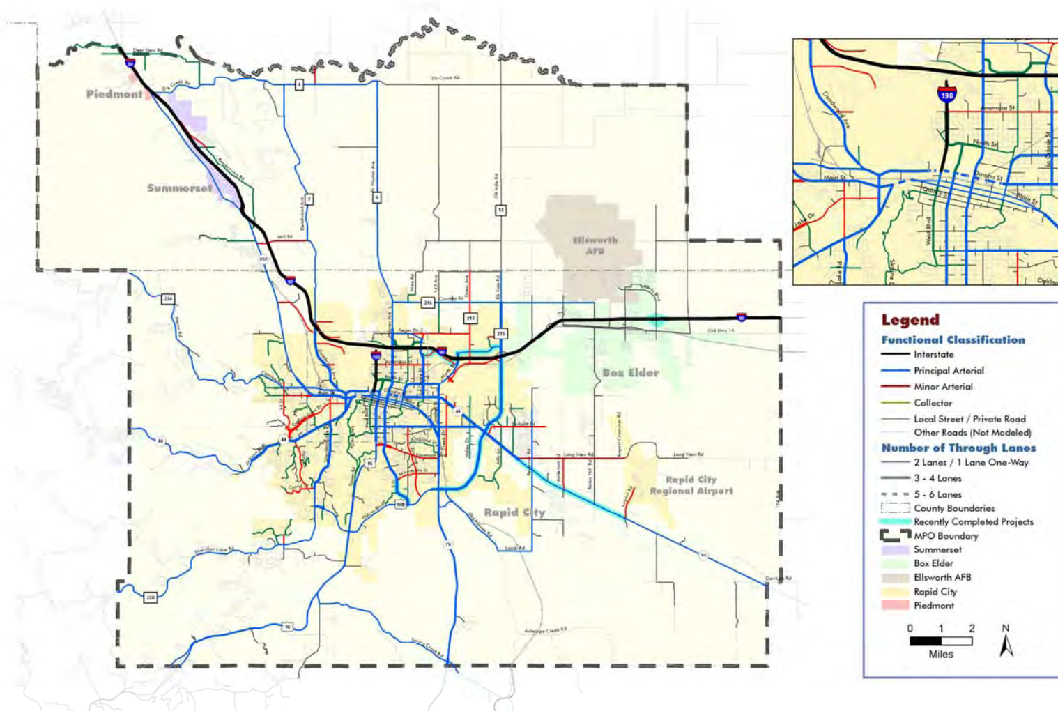
Figure 7-1: Existing Roadway System (2008) with Recently Completed Projects
