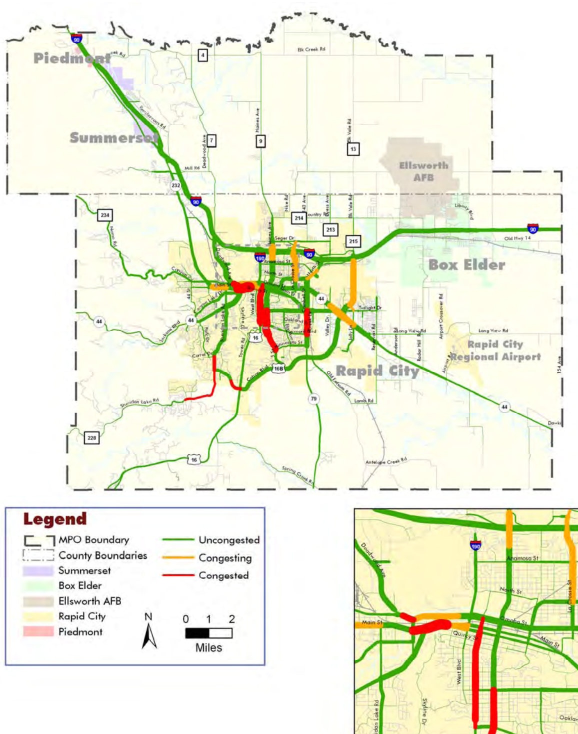
Figure 7-4: Needs Assessment – Roadway Congestion with 2035 Traffic on the 2013 Existing and Committed Network
