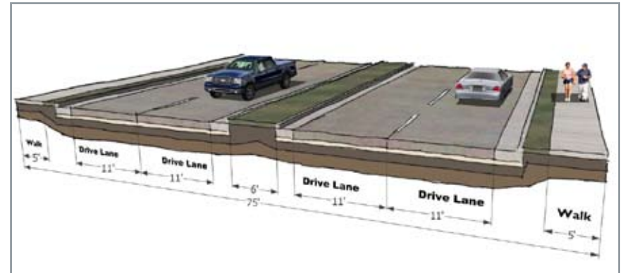
Proposed Section: 95'-100' Right-of-way, St. Patrick Street to Omaha Street
