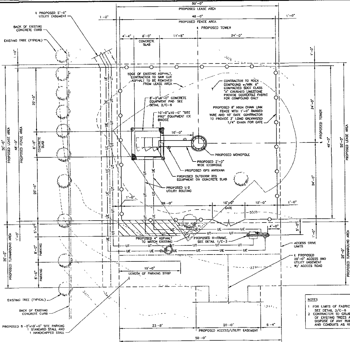
1 COMPOUND PLAN SCALE 3/16" = 1'-0"
