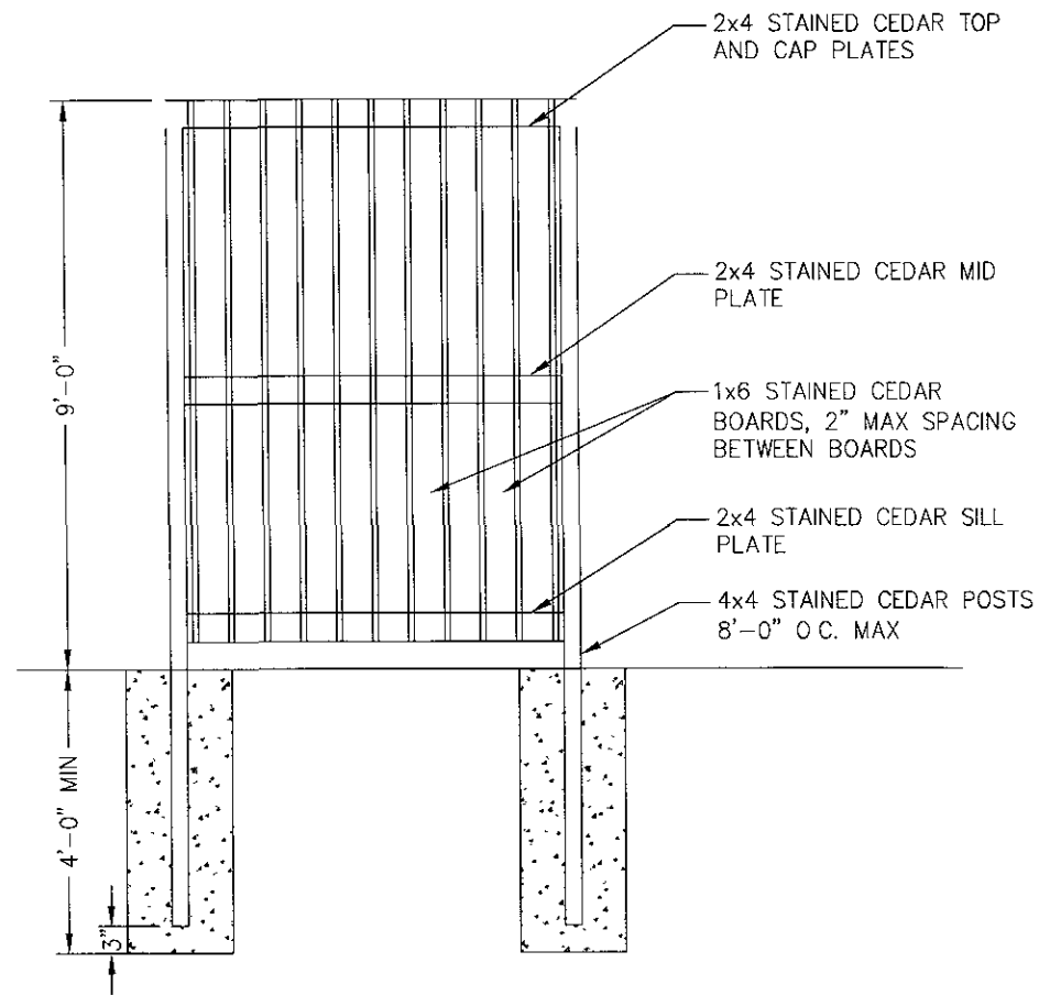
B FENCE ELEVATION SCALE: NONE
