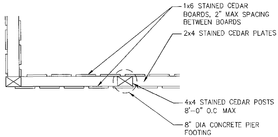
A PARTIAL PLAN SCALE: NONE
