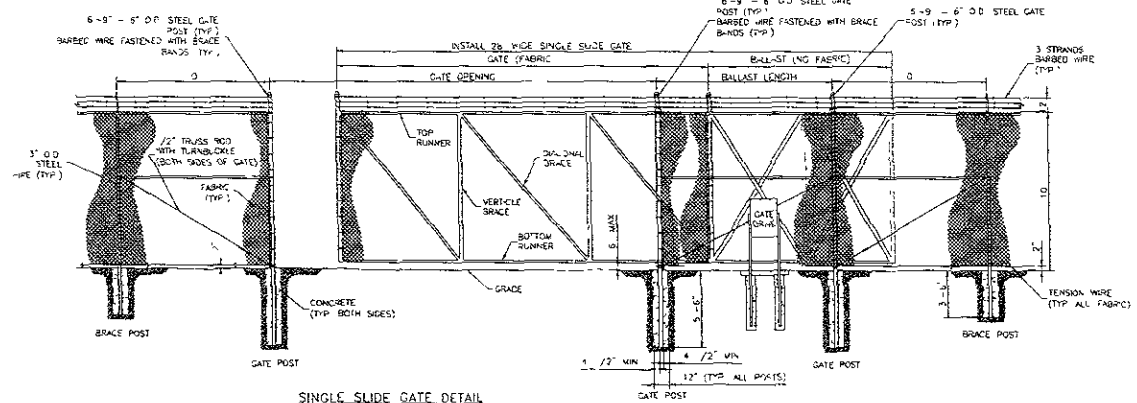
SINGLE SLIDE GATE DETAIL NOT TO SCALE
