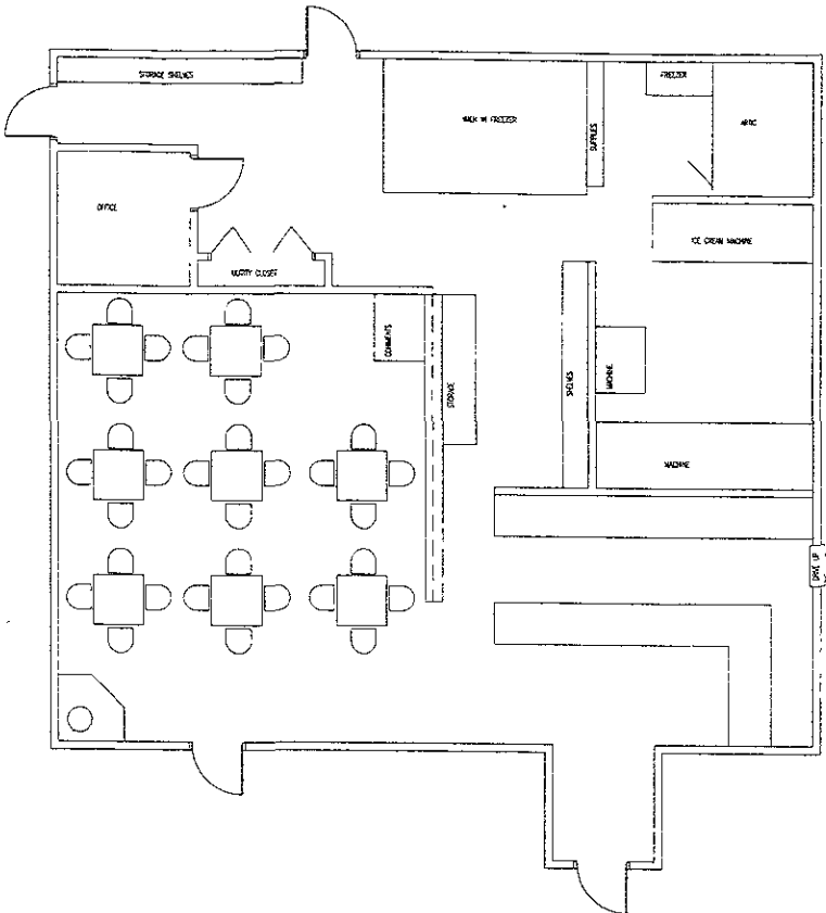
CONCEPTUAL FLOOR PLAN - GENERAL 1/8"=1'-0"
