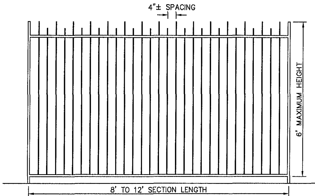
TYPICAL FENCE SECTION
