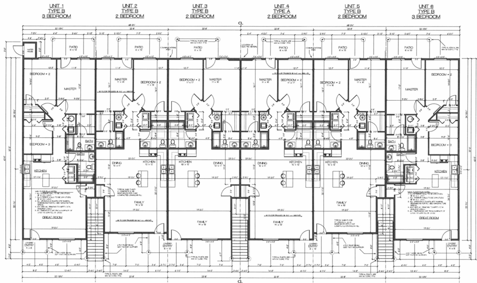
MAIN FLOOR PLAN SCALE: 3/8" = 1'-0"
