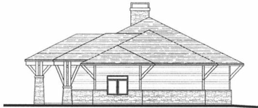
NORTH ELEVATION 1/8" = 1'-0"
