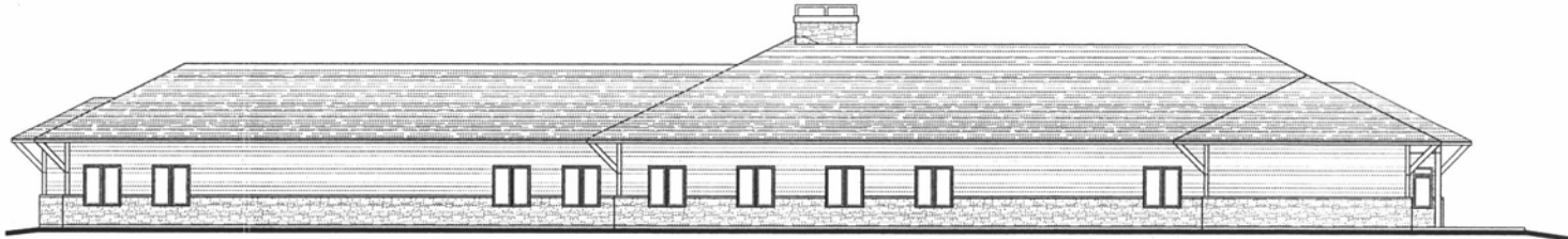
WEST ELEVATION 1/8" = 1'-0"
