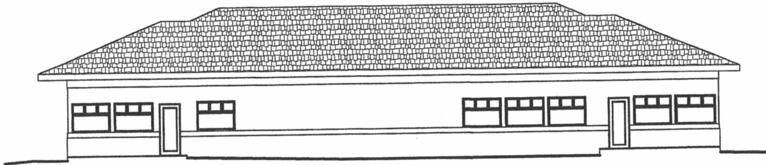
EAST ELEVATION
