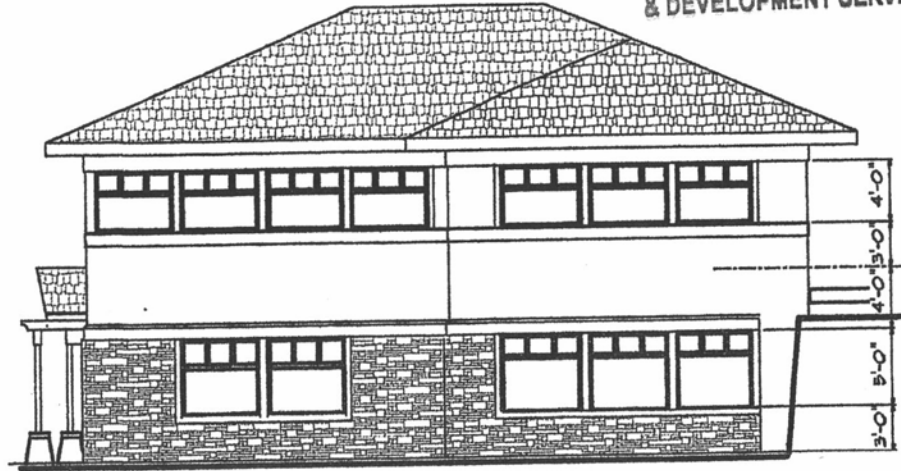
SOUTH ELEVATION
