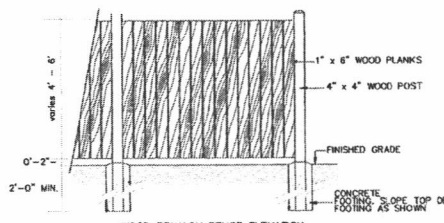
WOOD PRIVACY FENCE ELEVATION NOT TO SCALE NOT FOR CONSTRUCTION
