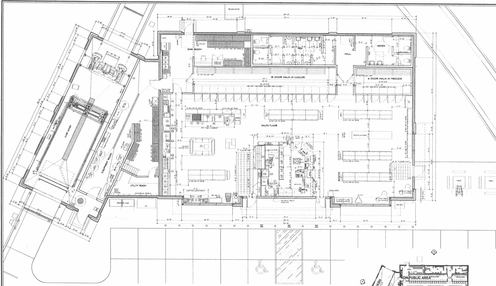
1 FLOOR PLAN 3/16" = 1'-0"
