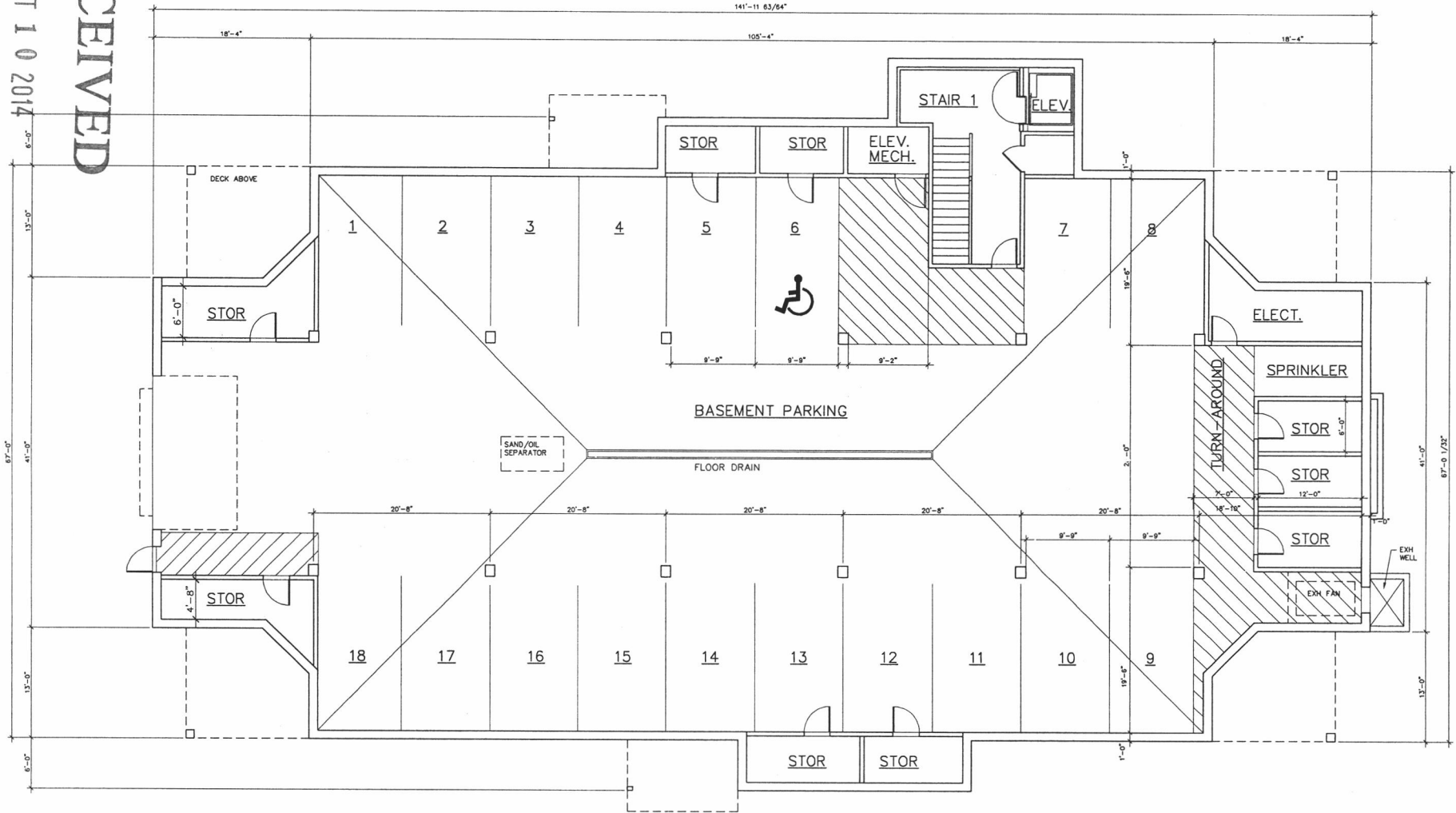
PROPOSED BASEMENT FLOOR PLAN #2 TOTAL BLDG. AREA: 9,258.0 SQ. FT. 3/16" = 1'-0"
