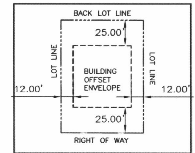
TYPICAL LOT DIMENSION
