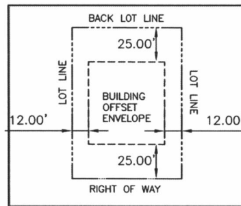
TYPICAL LOT DIMENSION
