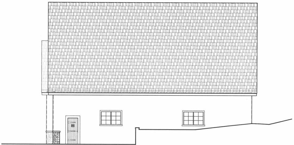
B RIGHT ELEVATION SCALE 3/8"=1'-0"
