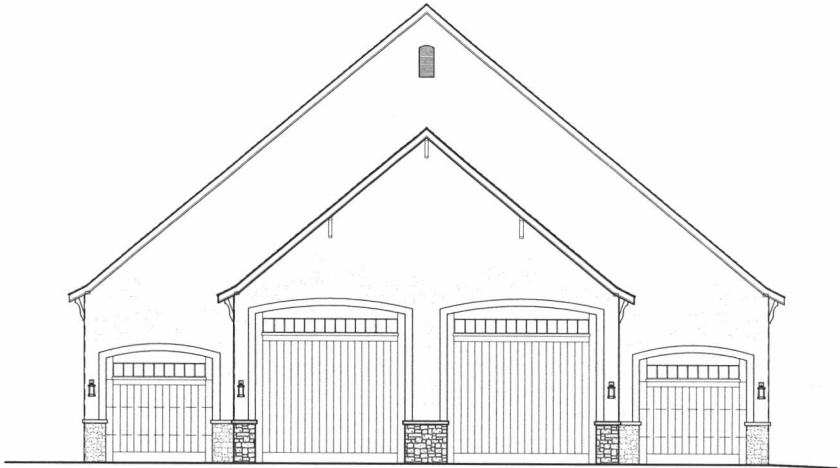
A FRONT ELEVATION SCALE 3/8"=1'-0"
