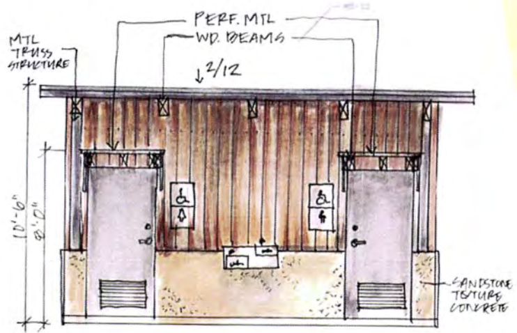
FRONT 1/4" = 1'-0"
