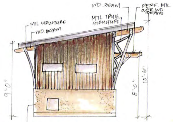
SANDSTONE TEXTURE CONCRETE LEFT 1/4" = 1'-0" LEFT SIDE ELEVATION
