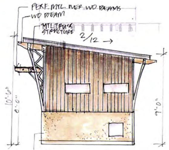
SANDSTONE TEXTURE CONCRETE RIGHT 1/4" = 1'-0"
