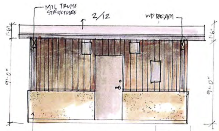
SANDSTONE TEXTURE CONCRETE REAR 1/4" = 1'-0" REAR ELEVATION
