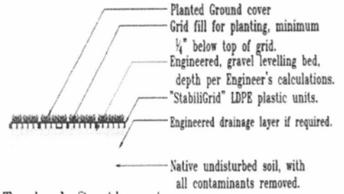
Typical Section A
