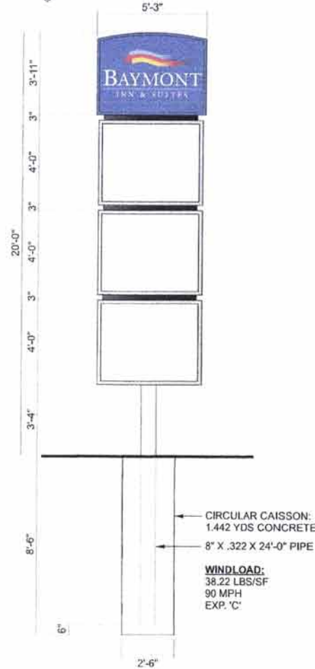
1 CUSTOM BAY-P20 - D/F Internally Illum'd Pylon Sign w/ additional Tenant Cabinets SCALE: 1/2"=1'-0"
