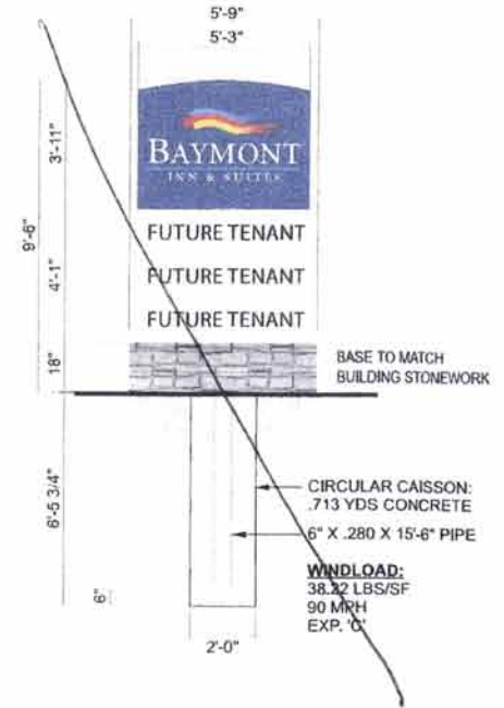
2 CUSTOM BAY-P20 - S/F Internally Illum'd Pylon Sign w/ additional Tenant Cabinets SCALE: 1/2"=1'-0"
