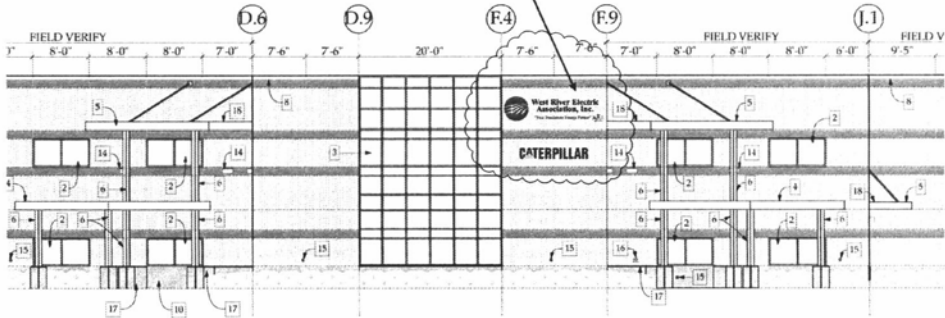
VIEW SOUTH ELEVATION
