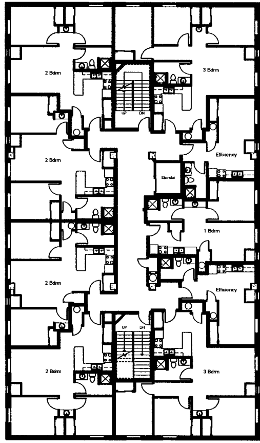
2 Floor Plan - Levels 2 - 6
