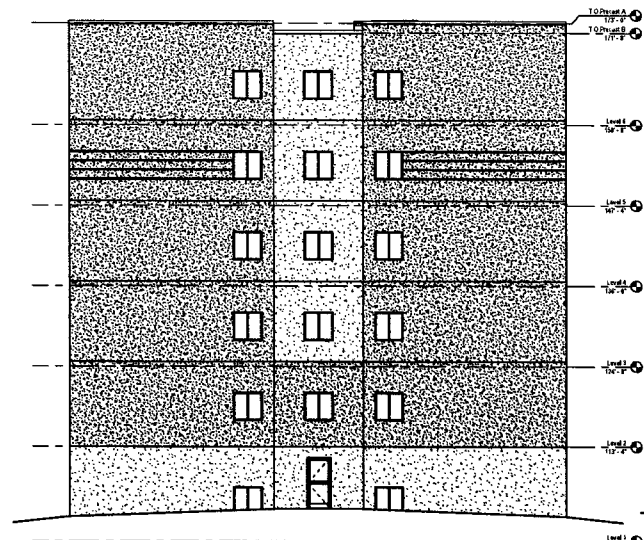
3 Elevation - South
