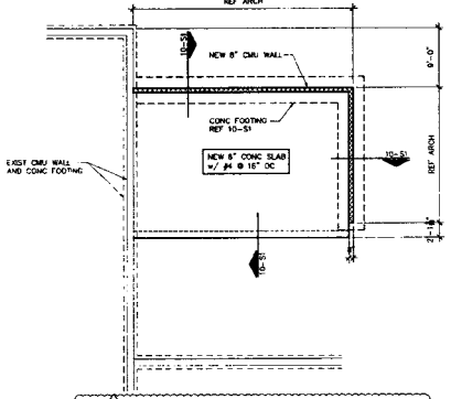
9 TIRE STORAGE SCREEN WALL SCALE: 1/8" = 1'-0"
