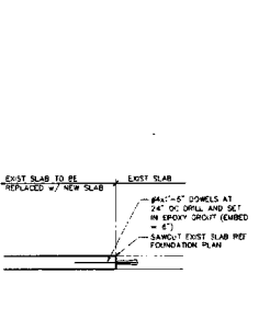
6 SLAB SAWCUT AT EXIST SCALE: 3/4" = 1'-0"
