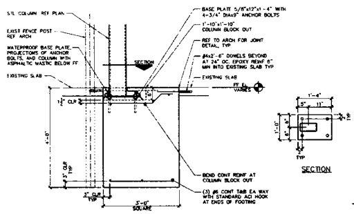
4 GARDEN CENTER CANOPY FOOTING SCALE: 3/4" = 1'-0"
