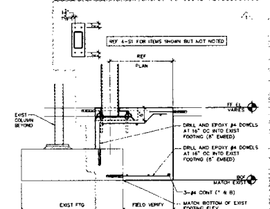
5 CANOPY FOOTING SCALE: 3/4" = 1'-0"
