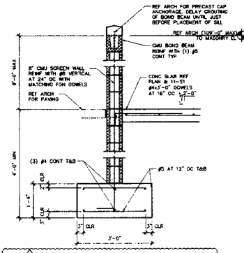
10 SCREEN WALL DETAIL SCALE: 3/4" = 1'-0"
