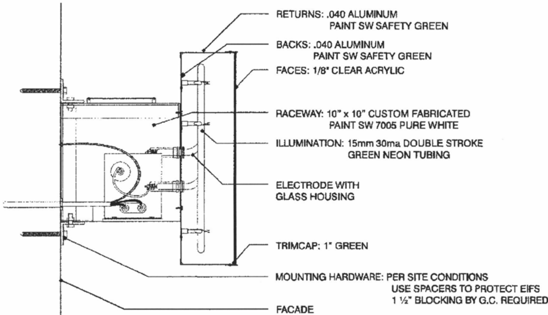
CC LETTER SECTION DETAIL SCALE: 1 1/2" = 1'
