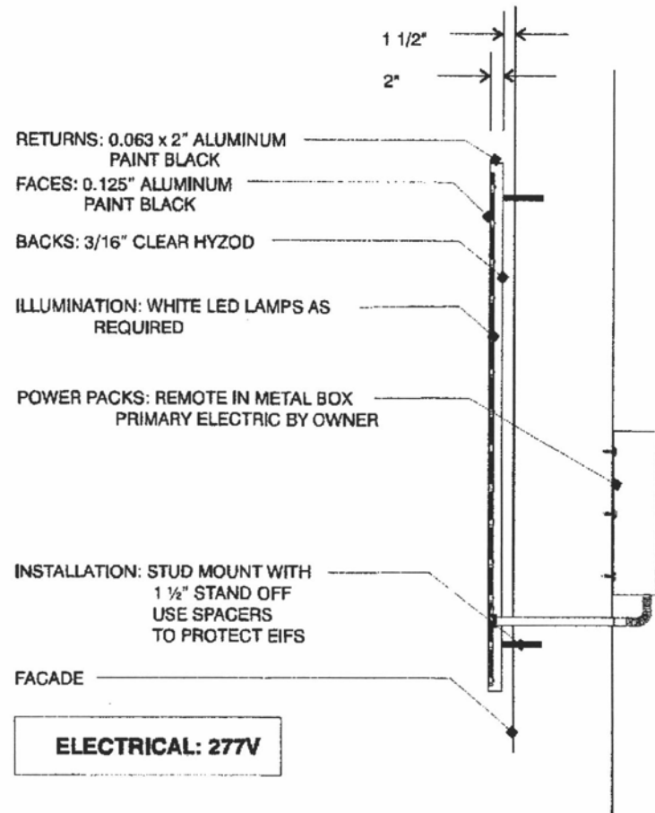
DD LETTER SECTION DETAIL SCALE: 1/2" = 1'
