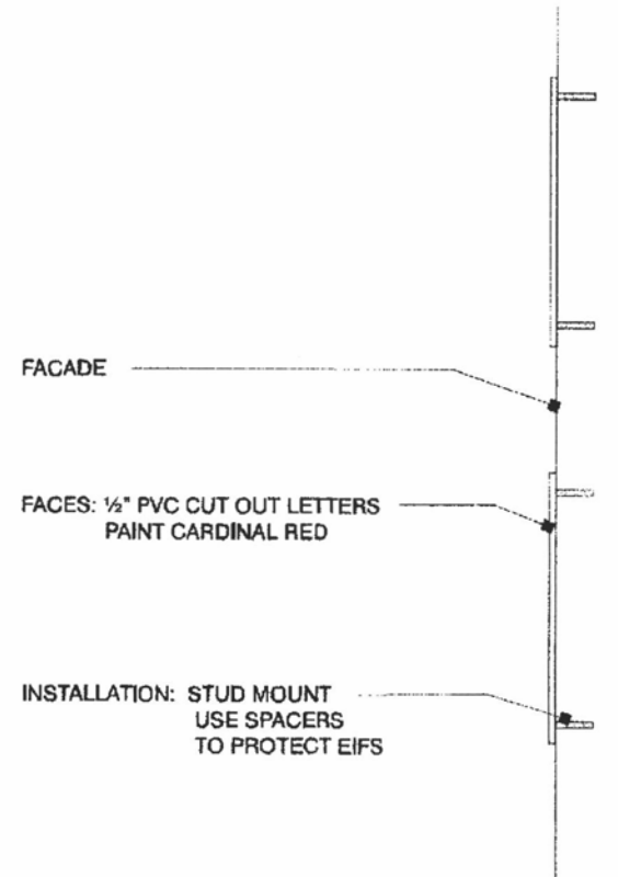
HH LETTER SECTION DETAIL SCALE: 3/4" = 1'
