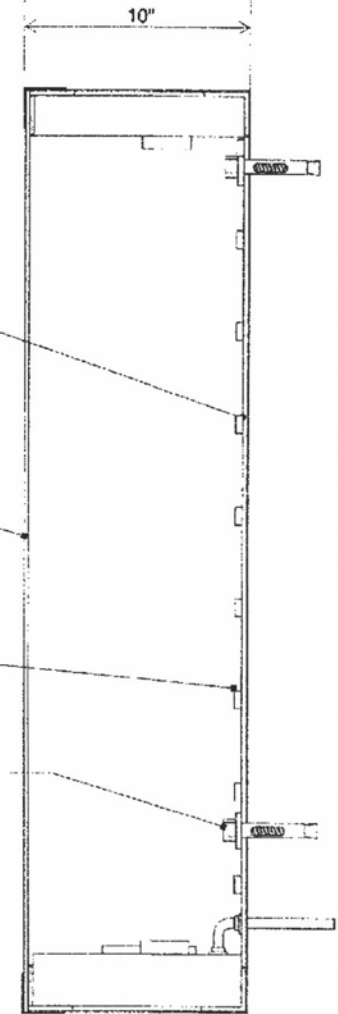
AA CABINET SECTION DETAIL SCALE: 1 1/2" = 1'
