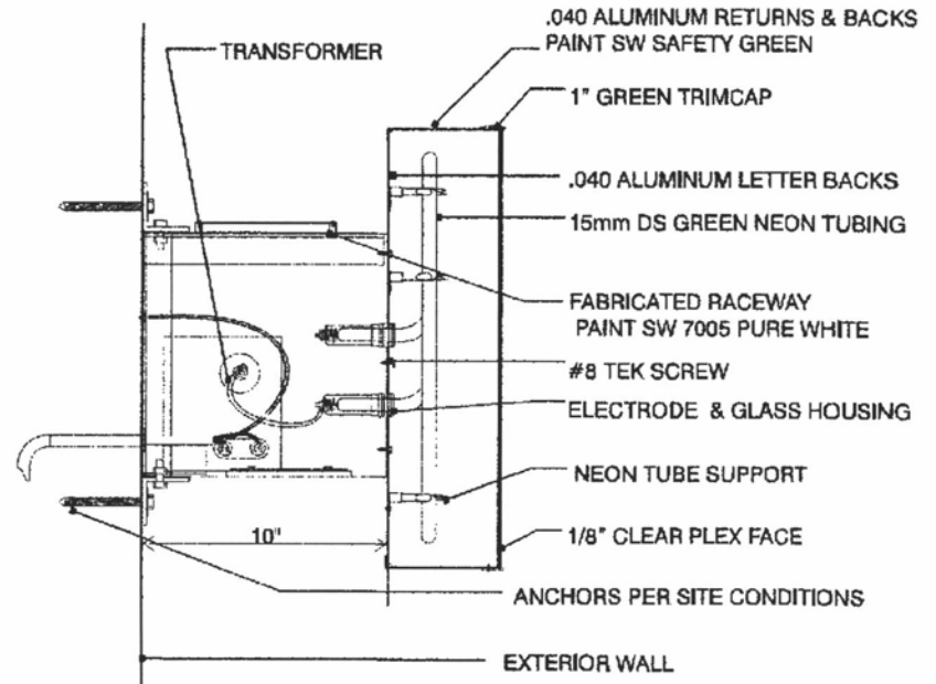
AA LETTER SECTION DETAIL SCALE: 1 1/2" = 1'
