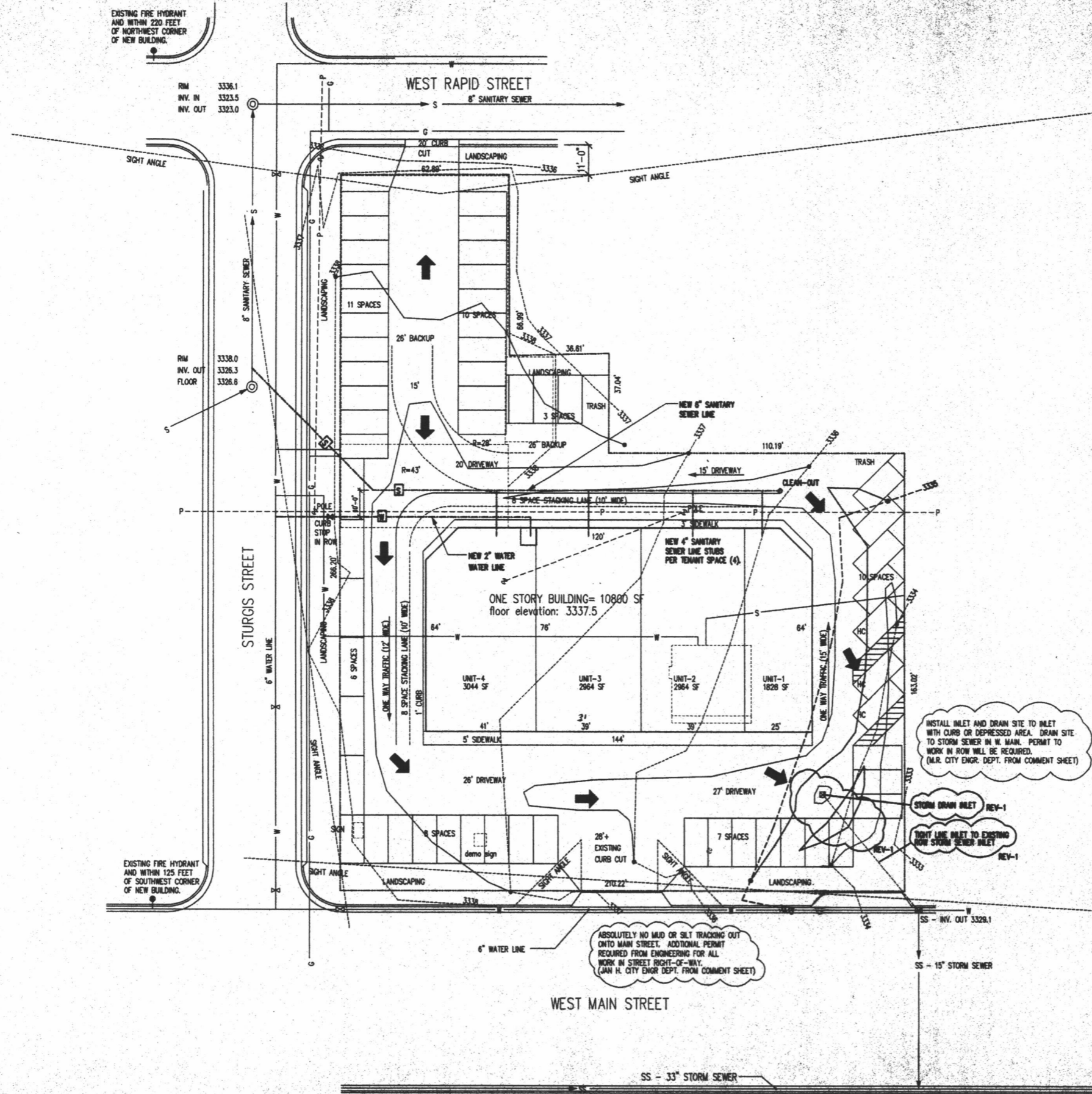
DRAINAGE/UTILITY PLAN SCALE: 1" = 20'
