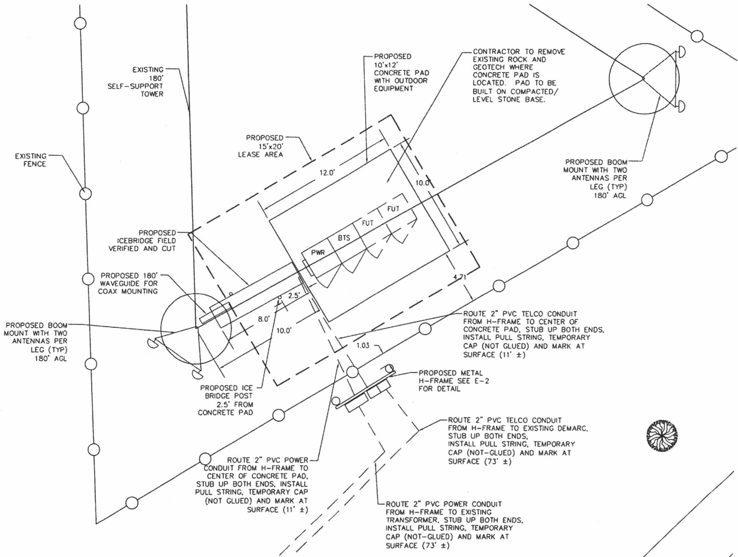
1 COMPOUND PLAN SCALE 1"=5'
