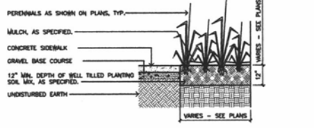
6 SECTION: PERENNIAL PLANTING BED DETAIL 19a SCALE: 1/2\"/>
