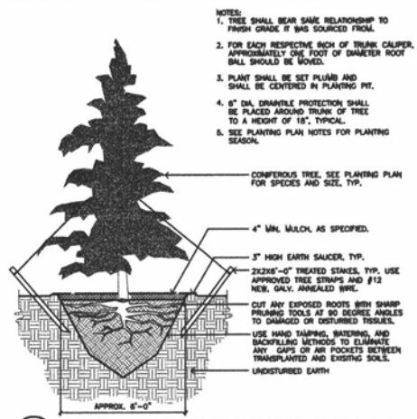
2 SECTION: 12' TRANSPLANTED CONIFEROUS TREE 19a NOT TO SCALE
