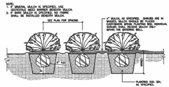
5 SECTION: TYPICAL SHRUB PLANTING BED 19a NO SCALE
