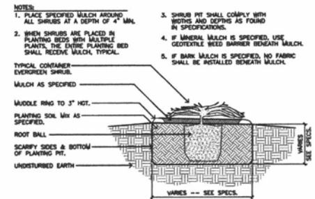
3 SECTION: CONTAINER CONIFEROUS SHRUB 19a NO SCALE
