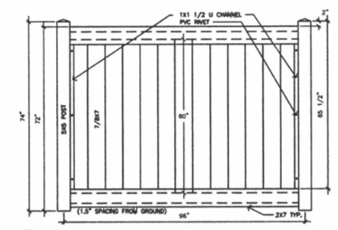
8 ELEVATION: 'LAKELAND' VINYL FENCE 19a SCALE: 3/4\"/>
