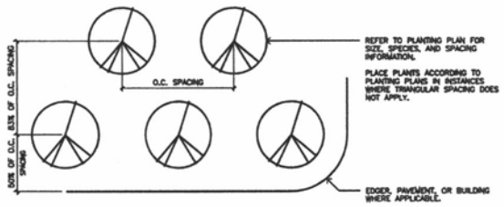
4 PLAN: TYPICAL TRIANGULAR SPACING PLANTING LAYOUT 19a NO SCALE
