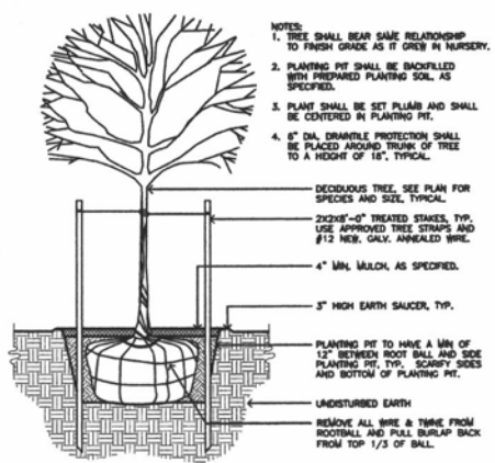
1 SECTION: TYPICAL B&B DECIDUOUS TREE 19a NO SCALE
