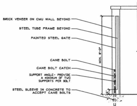
4 GATE SECTION AT TRASH ENCLOSURE SCALE: 1/2" = 1'-0"
