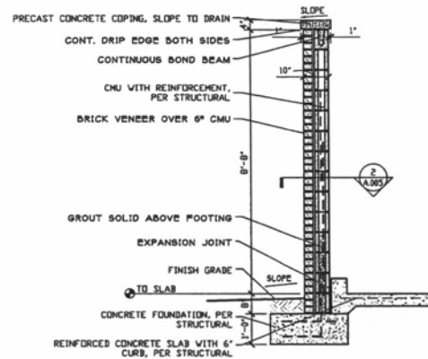
3 WALL SECTION AT TRASH ENCLOSURE SCALE: 1/2" = 1'-0"
