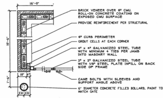
2 PLAN DETAIL - TRASH ENCLOSURE SCALE: 1/2" = 1'-0"
