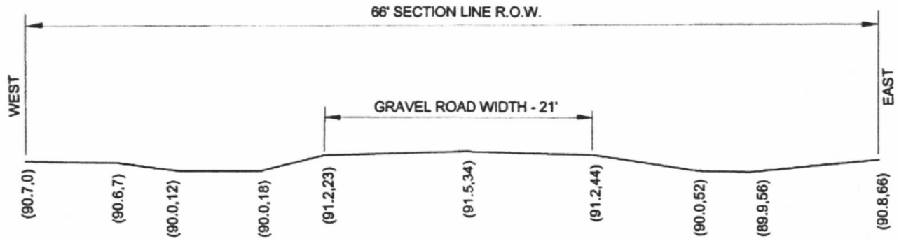
ROAD CROSS SECTION ON SECTION LINE
