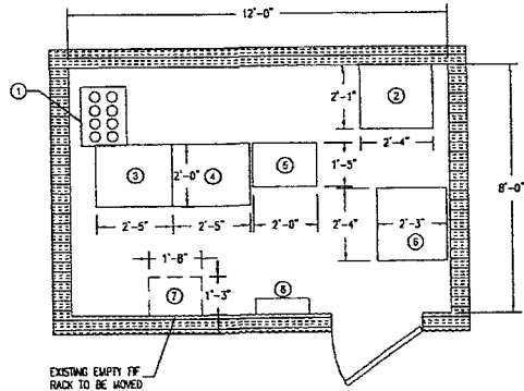
1 SITE PREPARATION LAYOUT SCALE: 1/4" = 1'-0"
