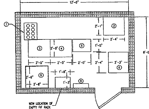
2 PROPOSED EQUIPMENT PLAN SCALE: 1/4" = 1'-0"
