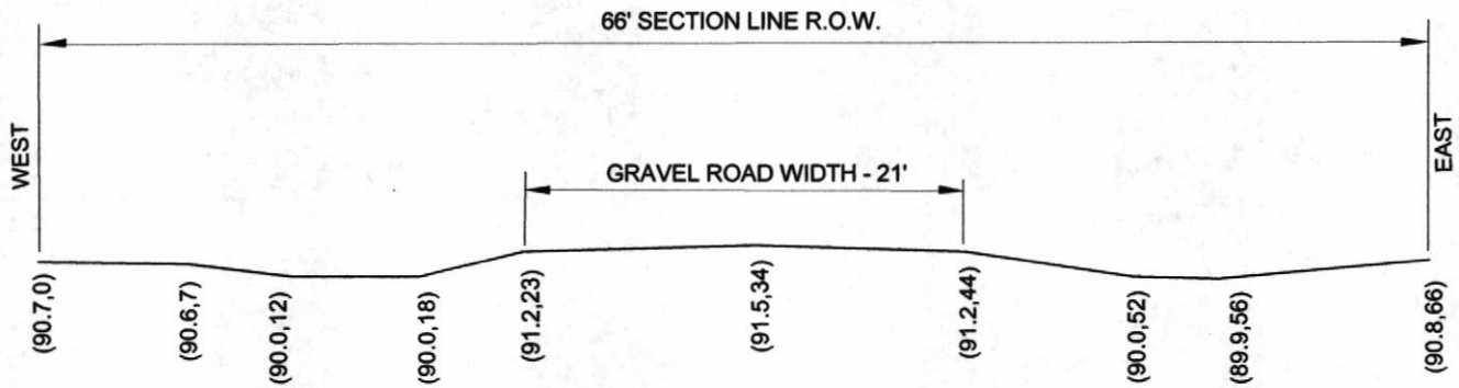
ROAD CROSS SECTION ON SECTION LINE
