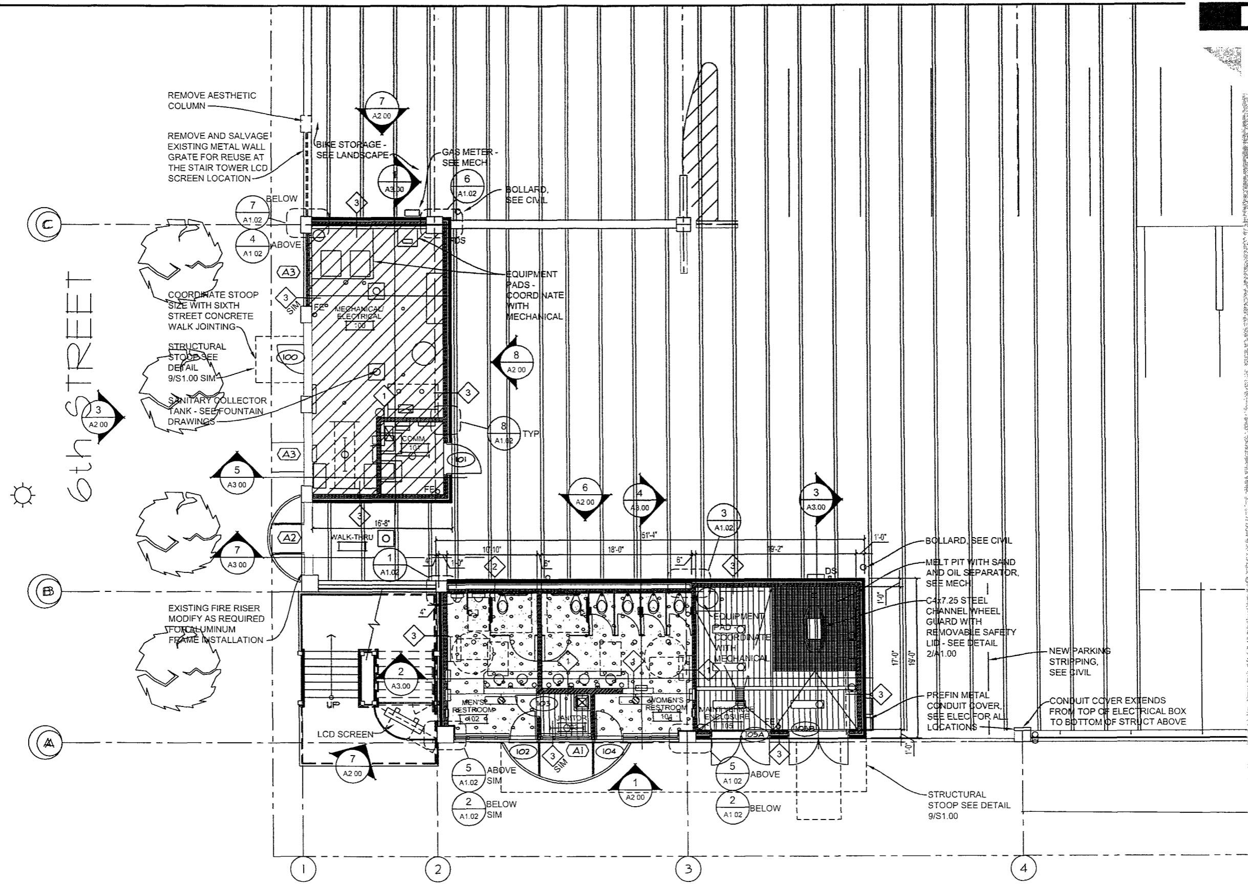
1 FLOOR PLAN A1.00 3/16" = 1' - 0"
