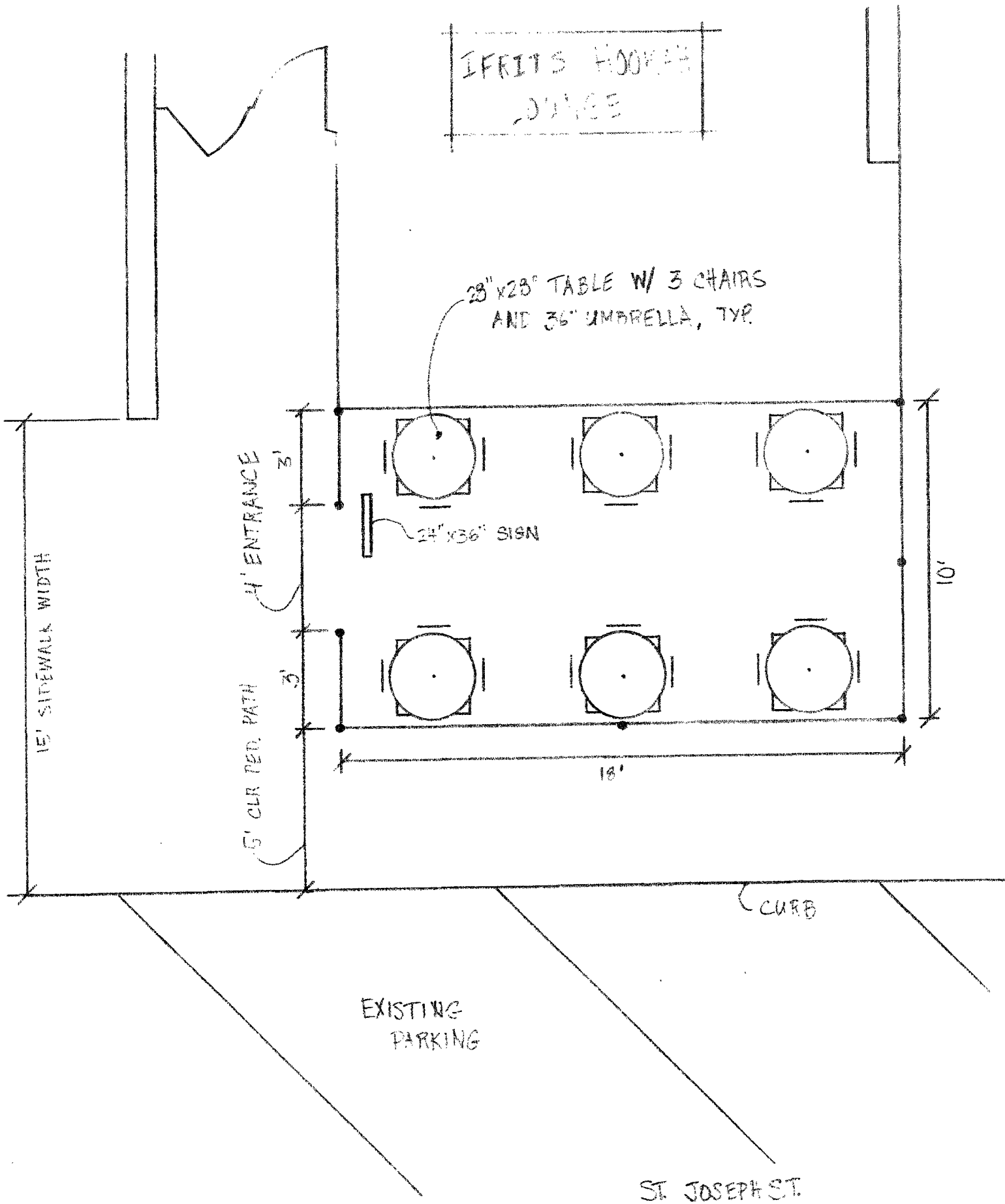
SIDEWALK PATIO SITE PLAN SCALE = 1/4" = 1'
