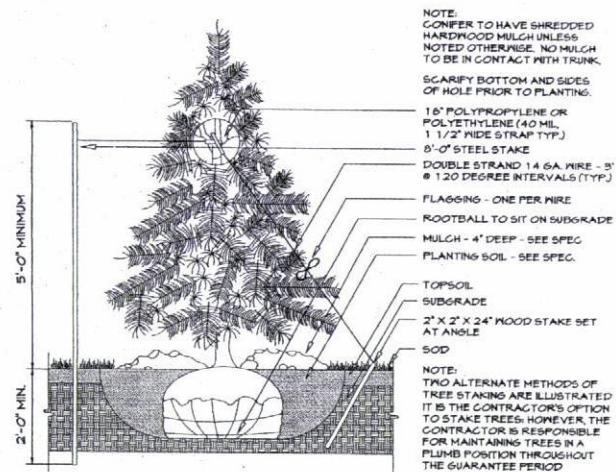
1 CONIFEROUS TREE IN MULCH N.T.S.
