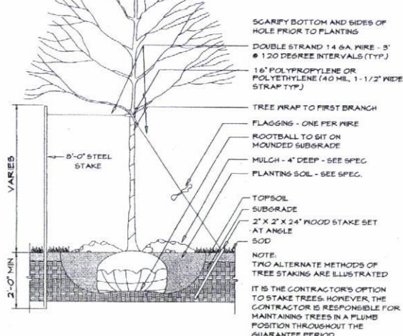
2 DECIDUOUS TREE IN MULCH N.T.S.
