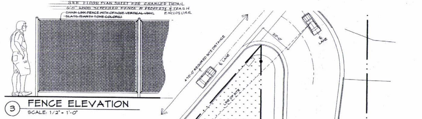
3 FENCE ELEVATION SCALE: 1/2" = 1'-0"
