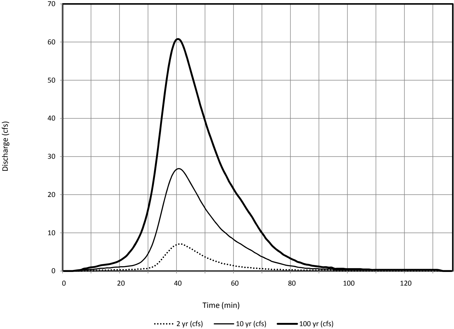
Subbasin 186 - DBDP Hydrologic Conditions
