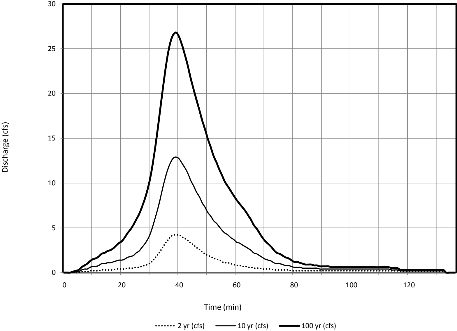
Subbasin 196 - DBDP Hydrologic Conditions
