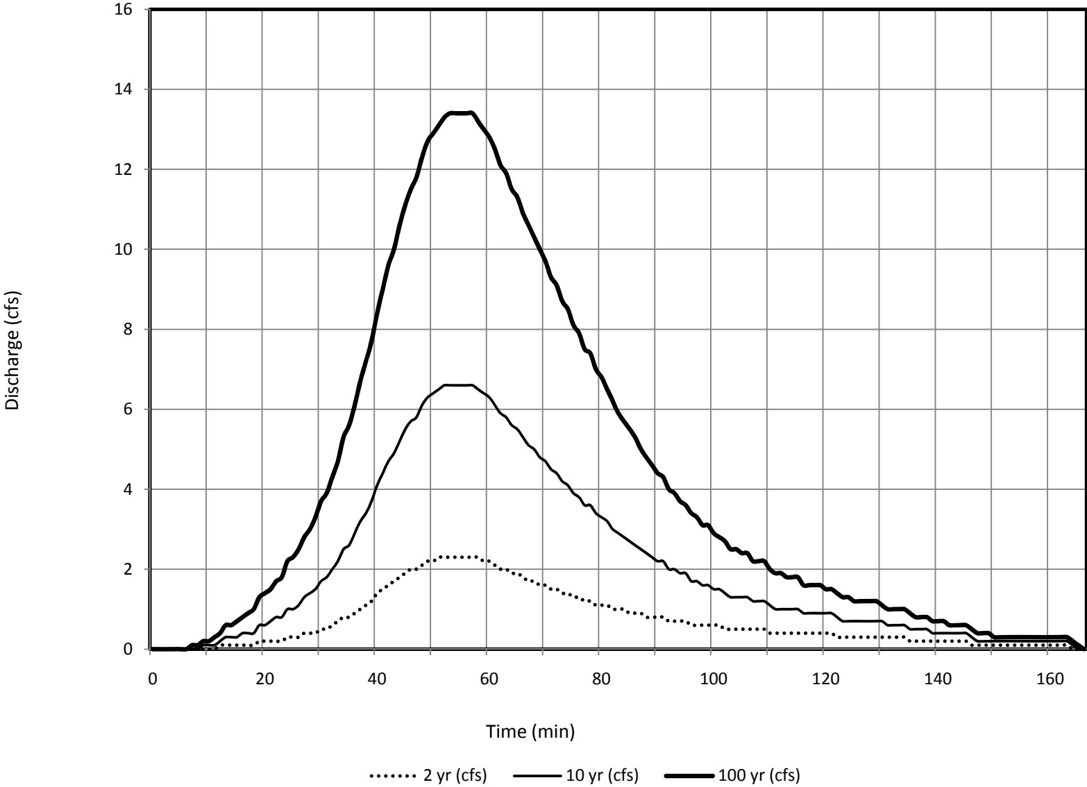
Subbasin 262 - DBDP Hydrologic Conditions
