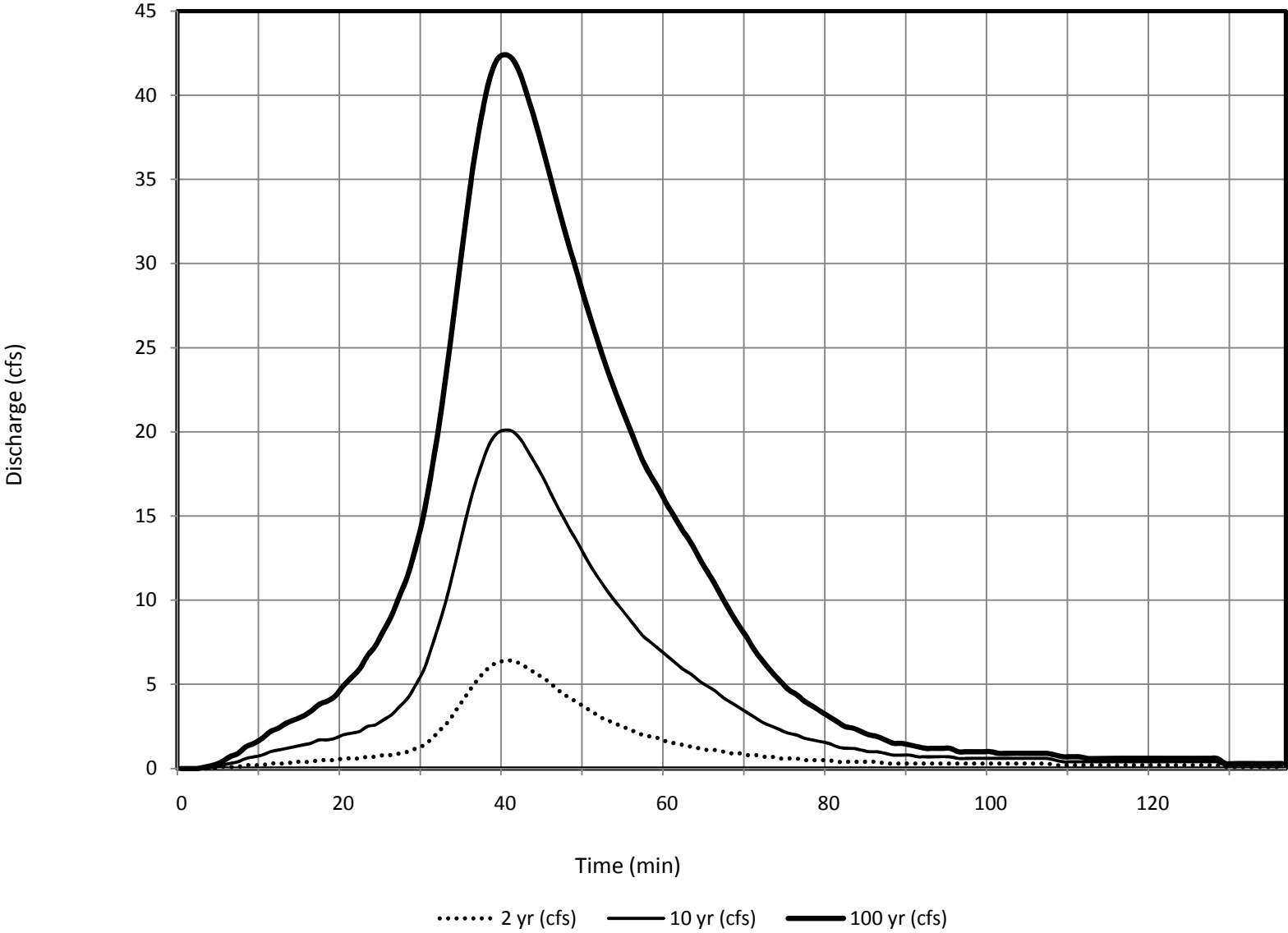
Subbasin 216 - DBDP Hydrologic Conditions
