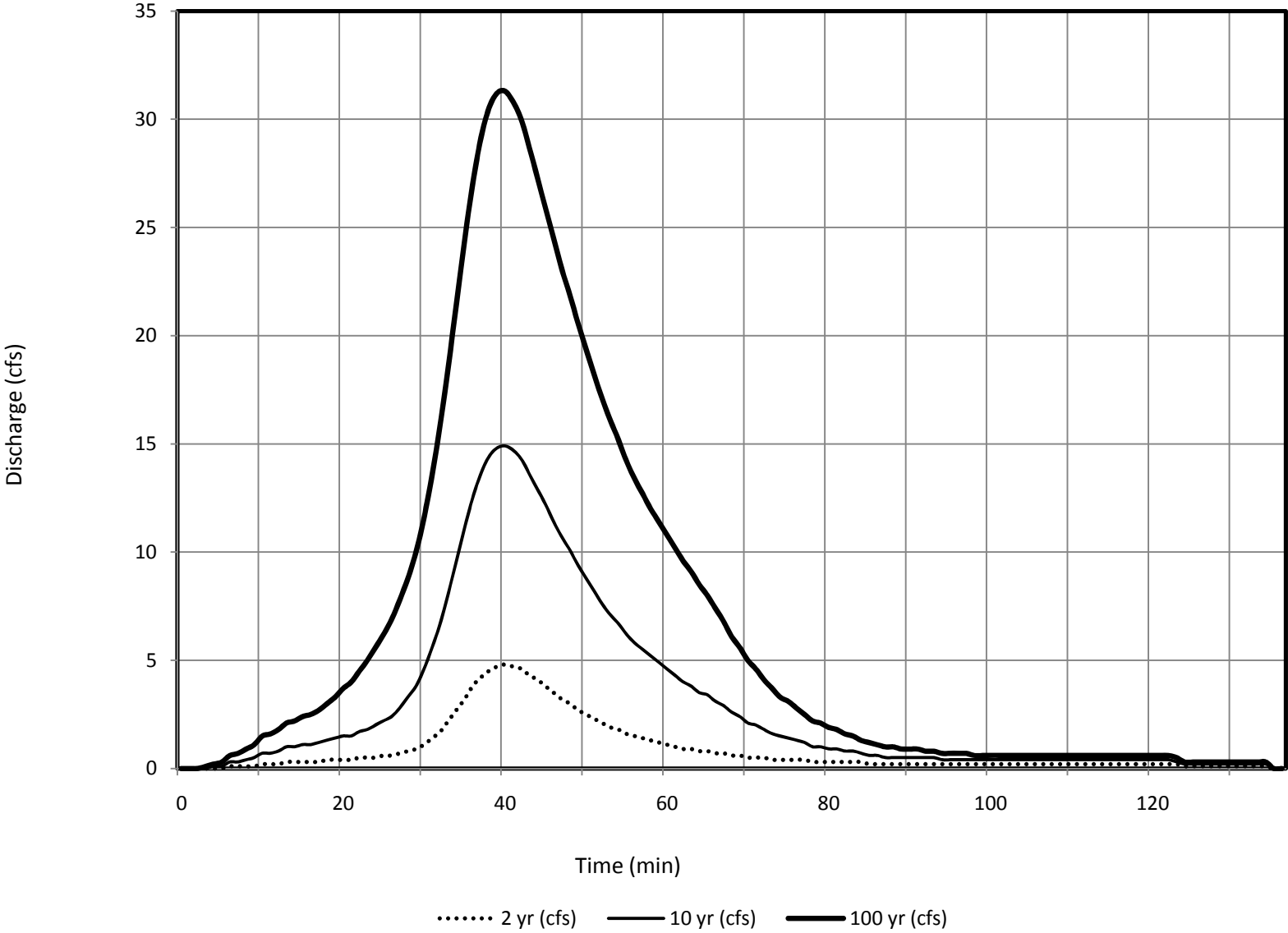
Subbasin 172 - DBDP Hydrologic Conditions
