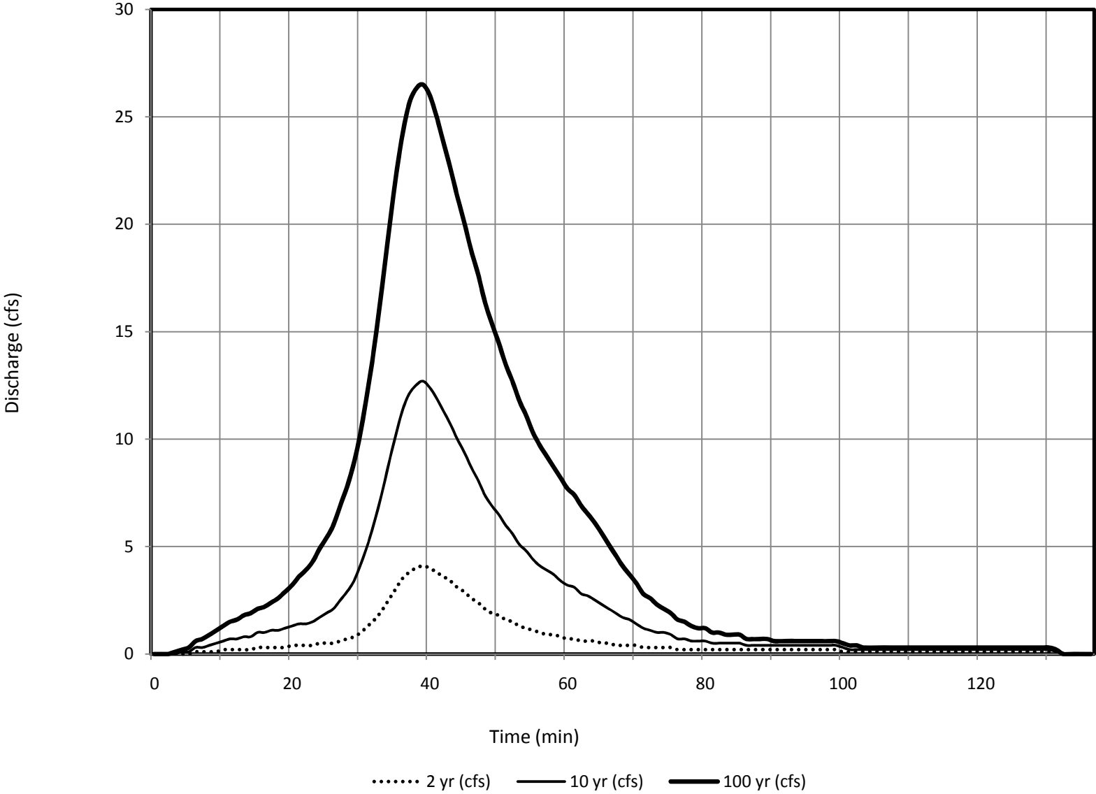
Subbasin 168 - DBDP Hydrologic Conditions
