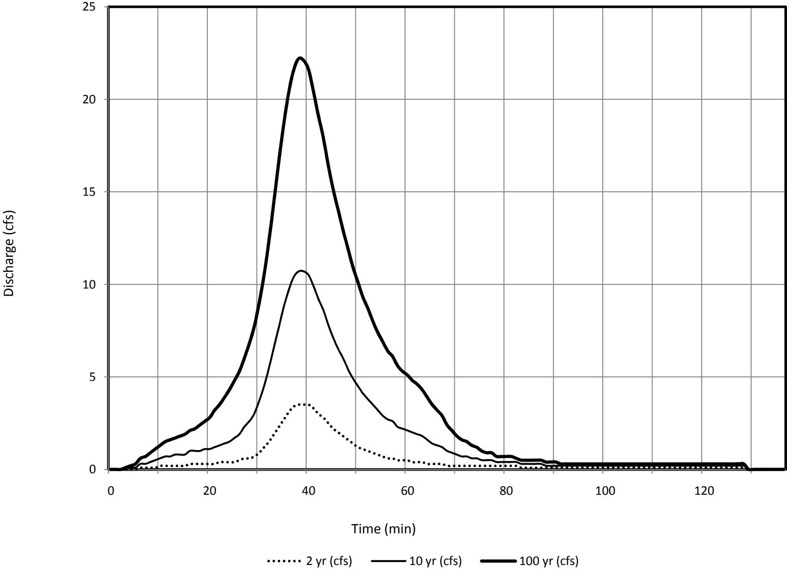
Subbasin 252 - DBDP Hydrologic Conditions
