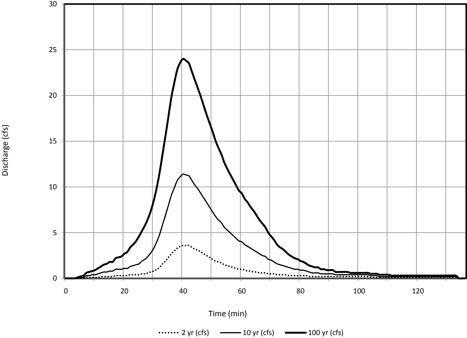
Subbasin 162 - DBDP Hydrologic Conditions
