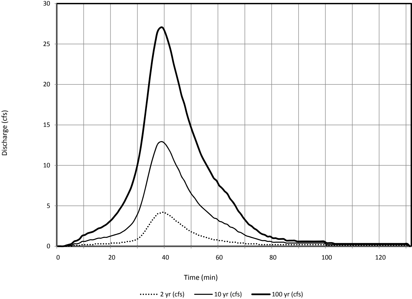
Subbasin 202 - DBDP Hydrologic Conditions
