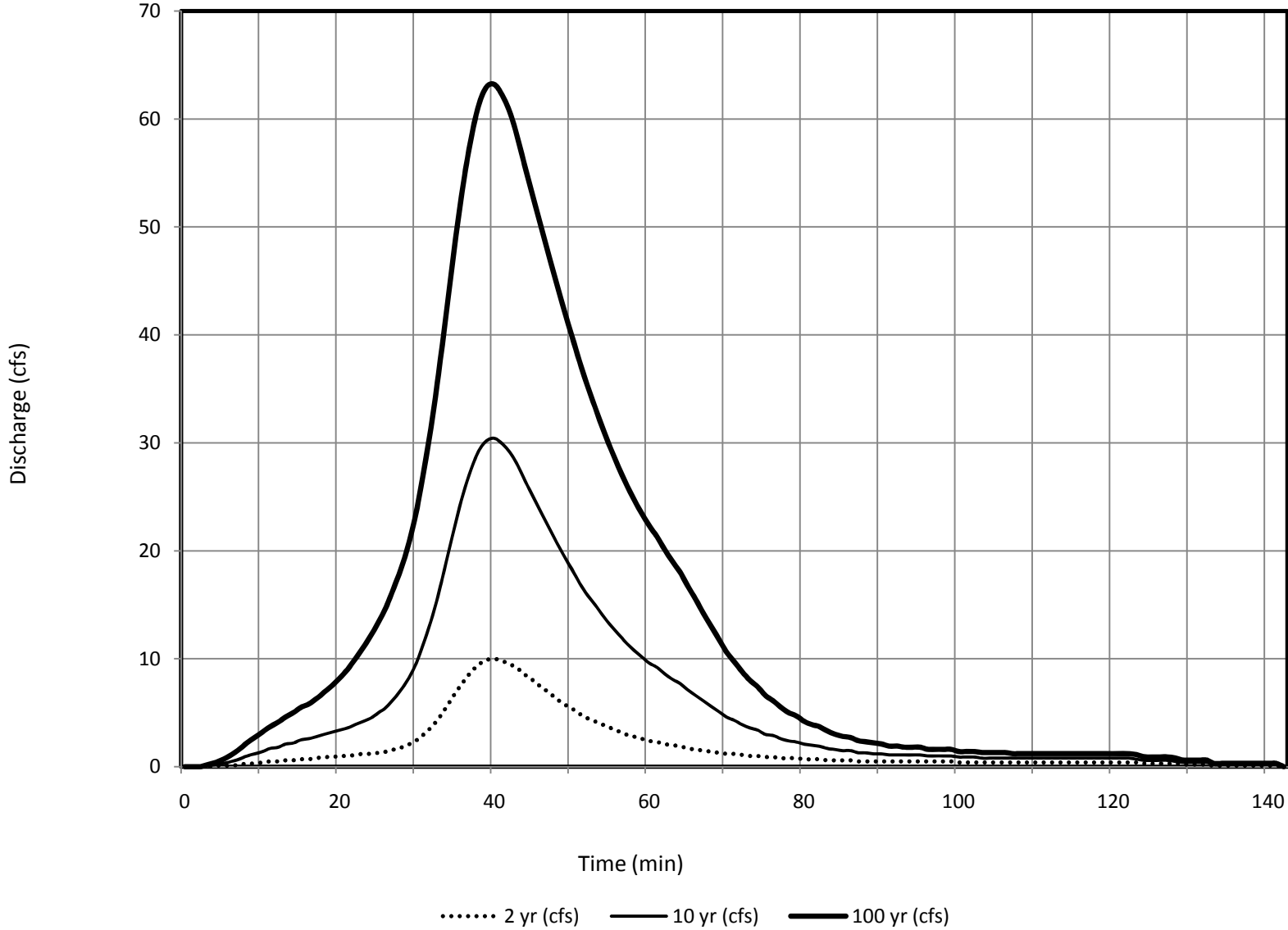
Subbasin 182 - DBDP Hydrologic Conditions
