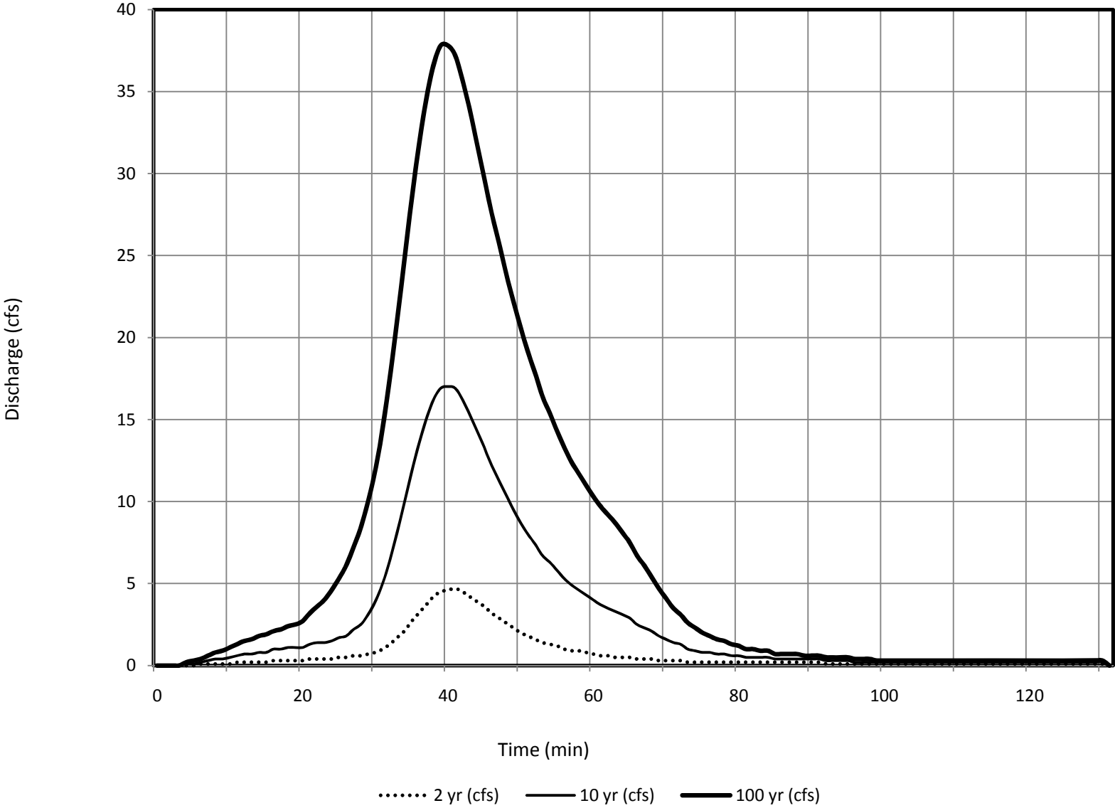
Subbasin 272 - DBDP Hydrologic Conditions
