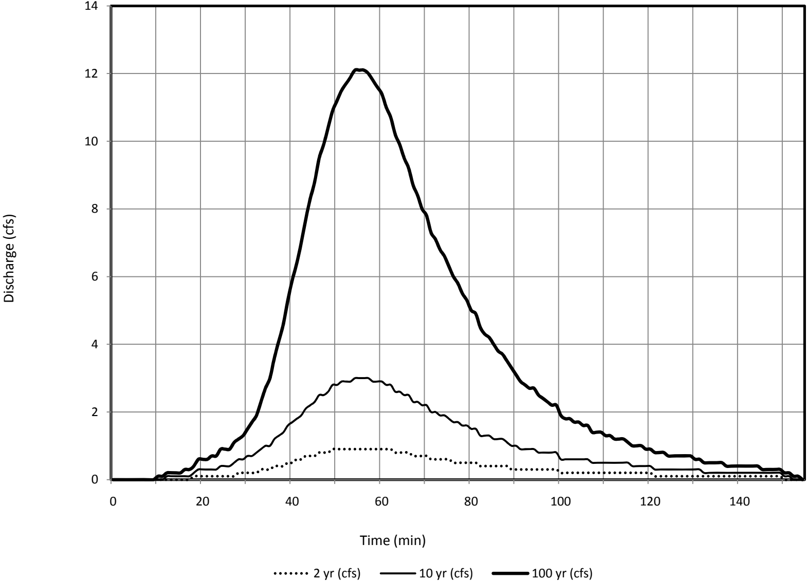
Subbasin 258 - DBDP Hydrologic Conditions
