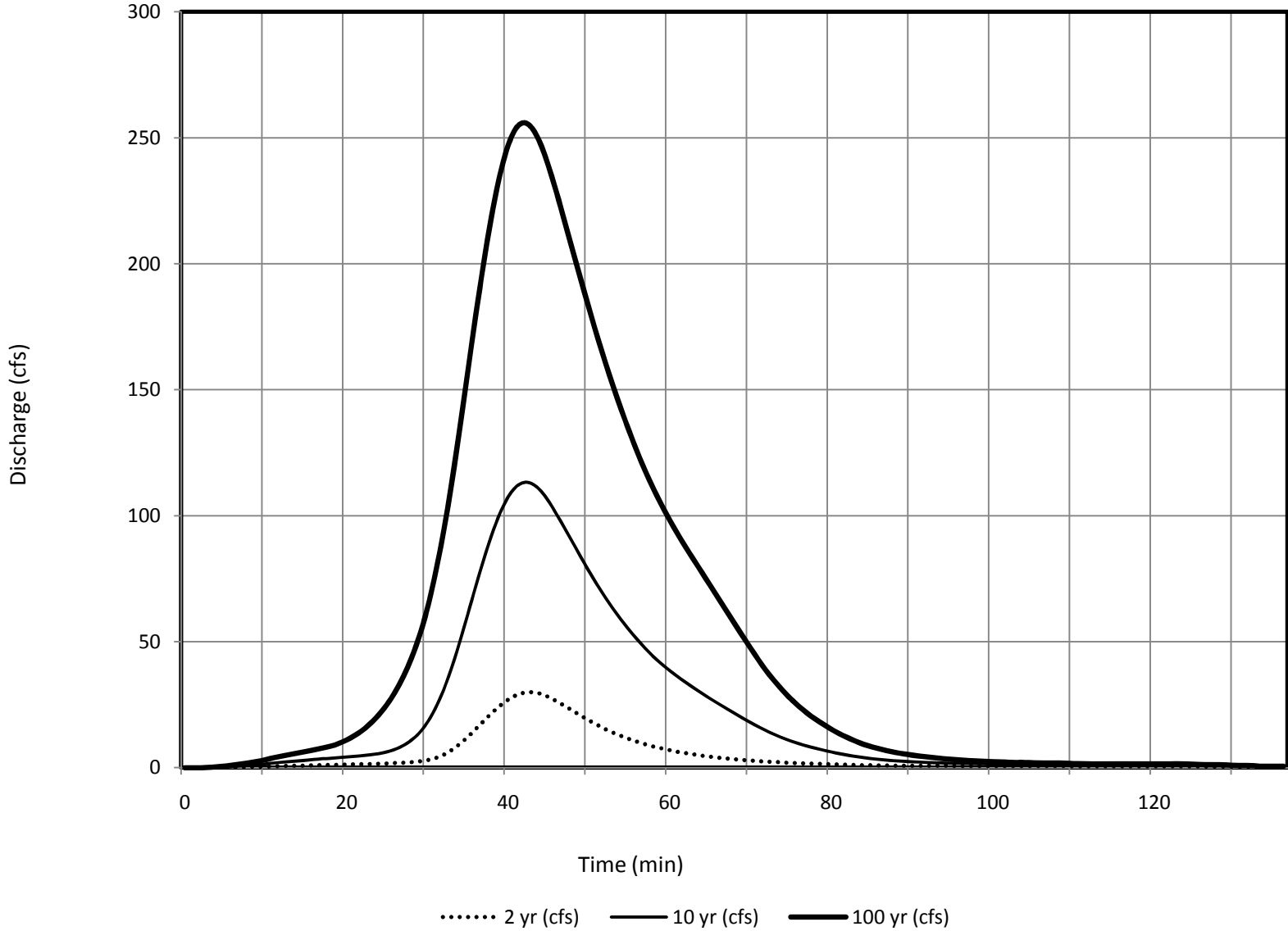
Subbasin 268 - DBDP Hydrologic Conditions
