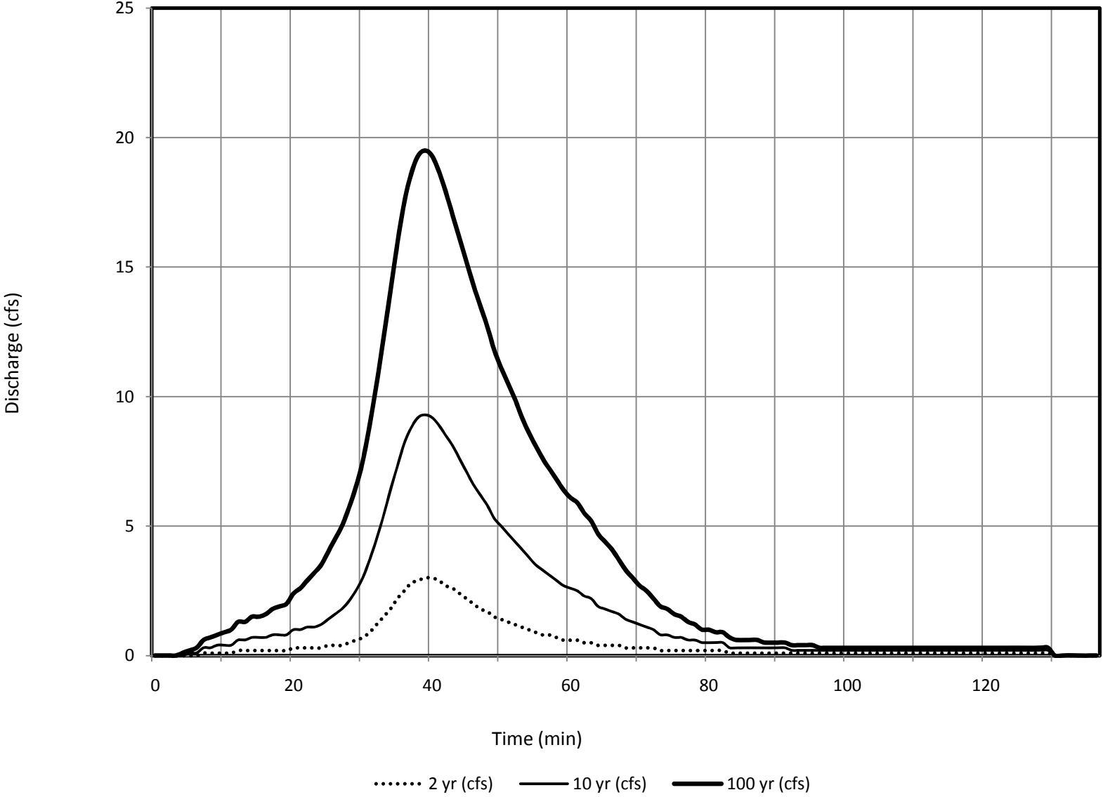
Subbasin 178 - DBDP Hydrologic Conditions
