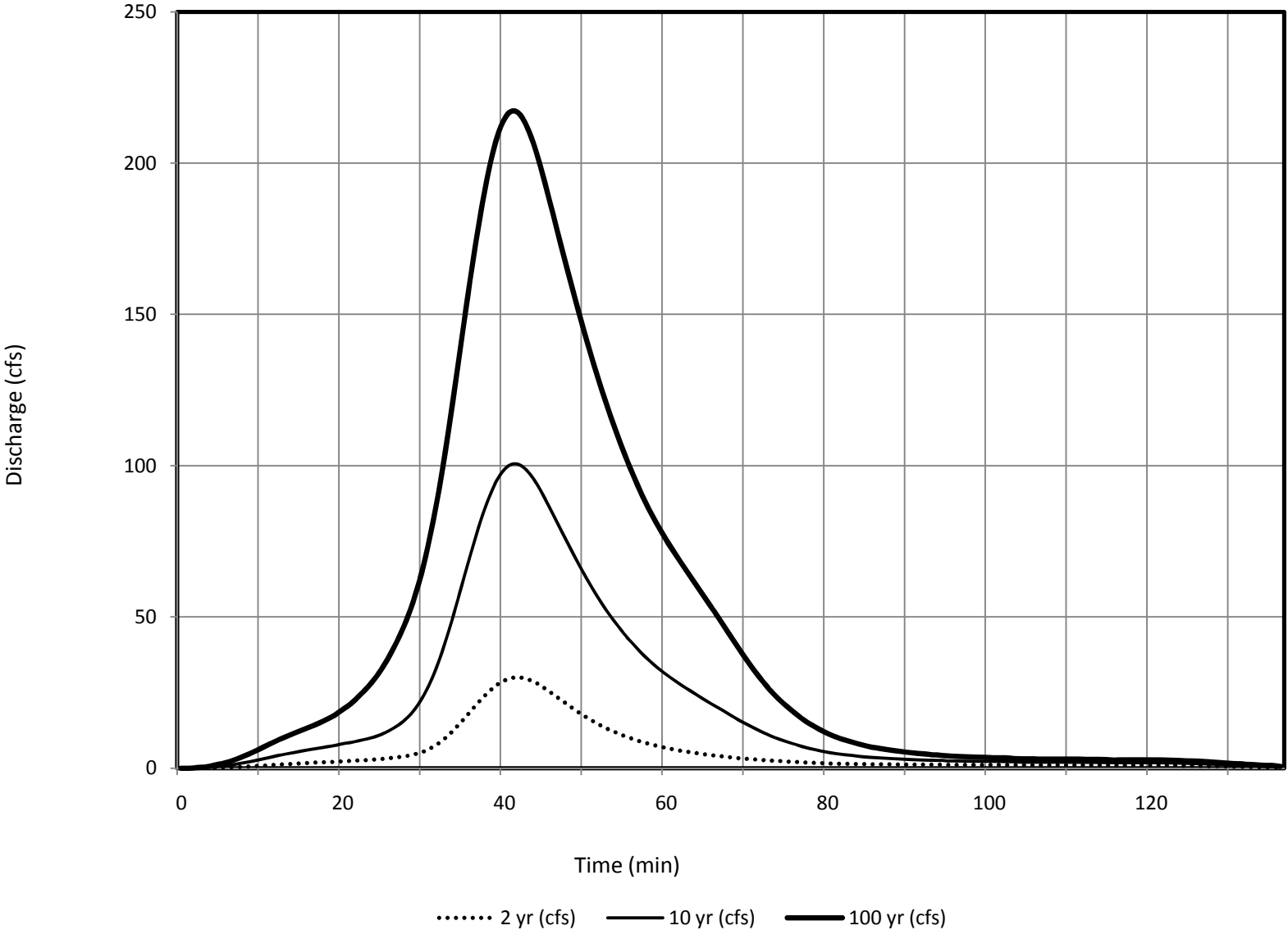
Subbasin 276 - DBDP Hydrologic Conditions
