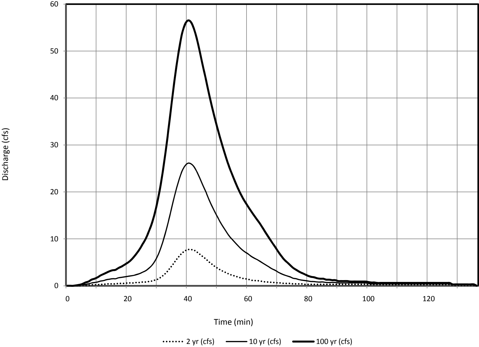
Subbasin 286 - DBDP Hydrologic Conditions
