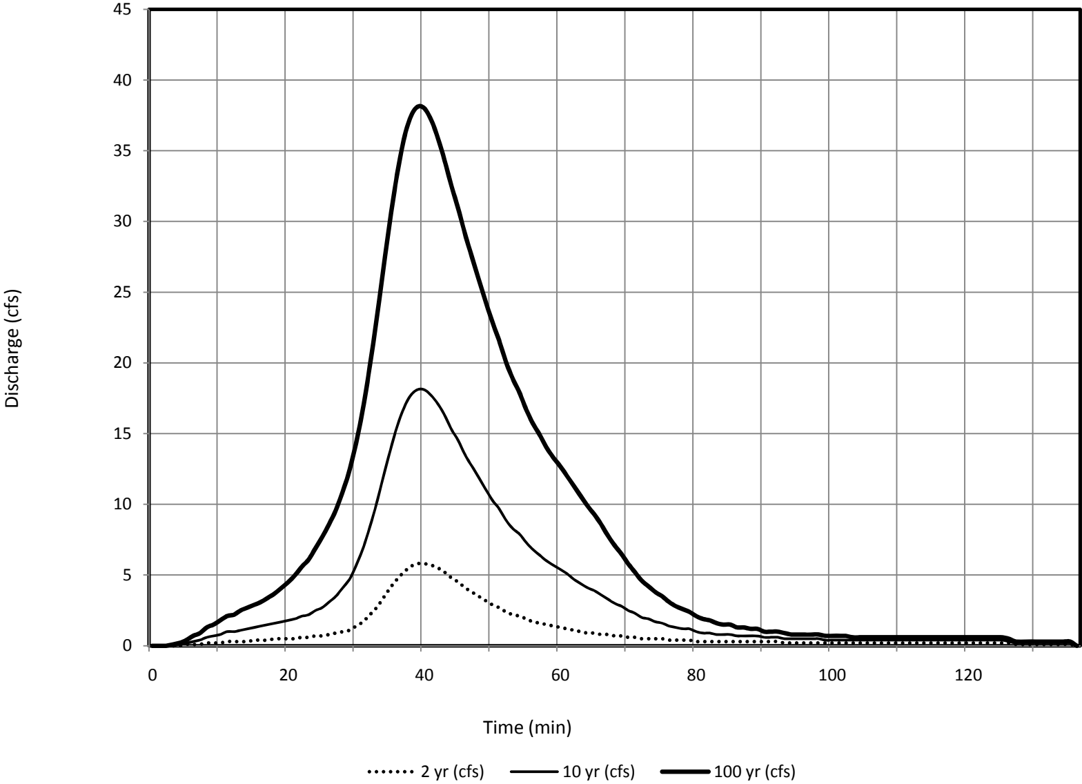
Subbasin 198 - DBDP Hydrologic Conditions
