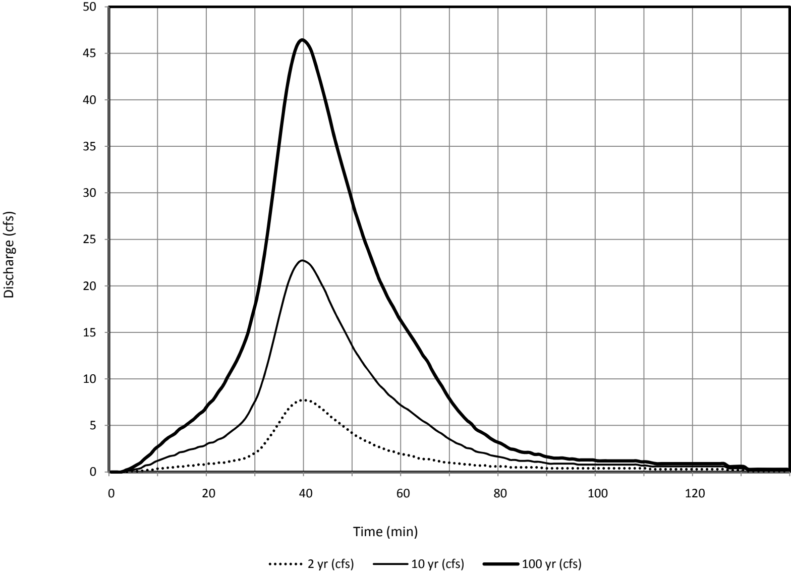
Subbasin 184 - DBDP Hydrologic Conditions
