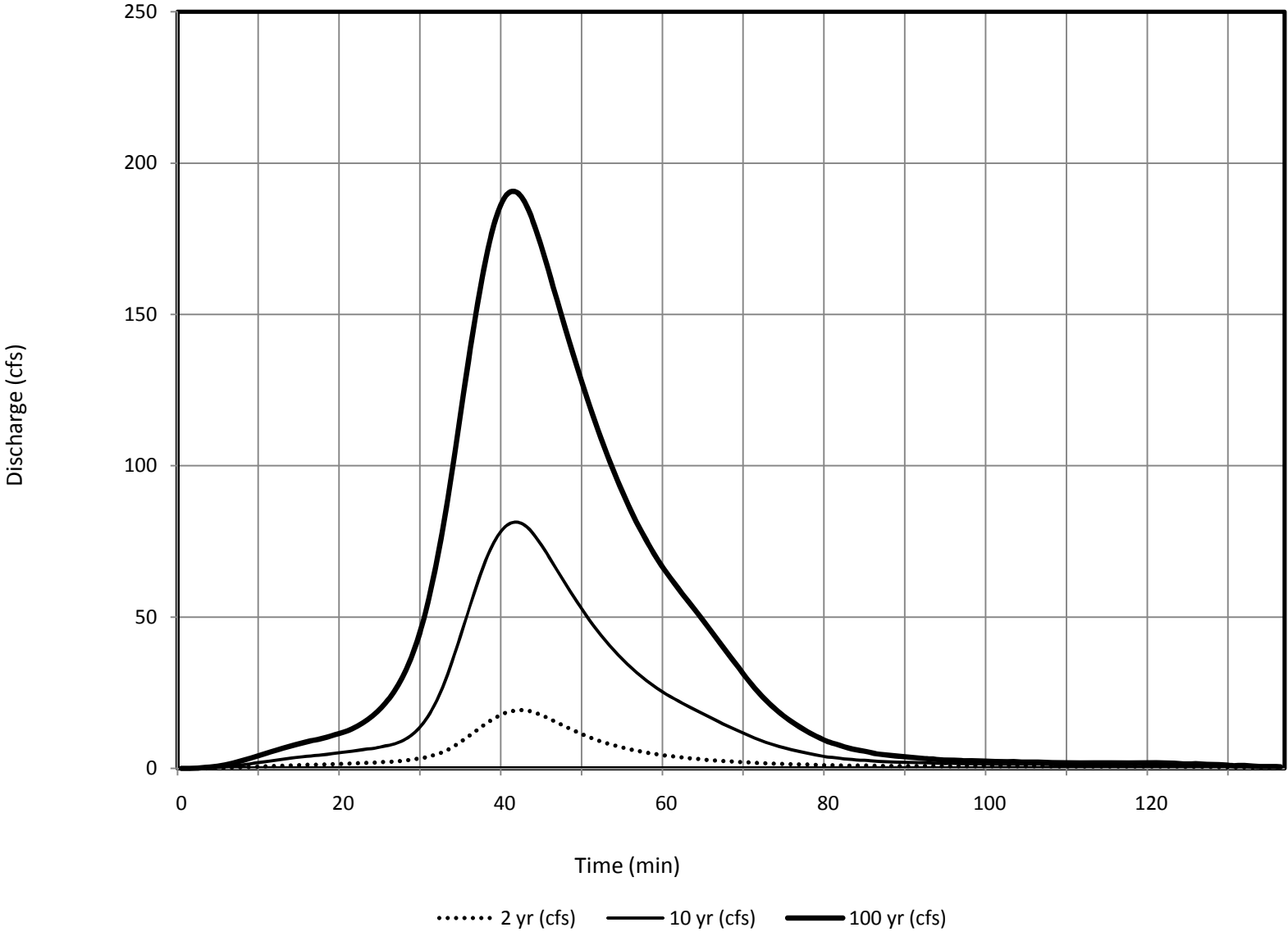
Subbasin 284 - DBDP Hydrologic Conditions
