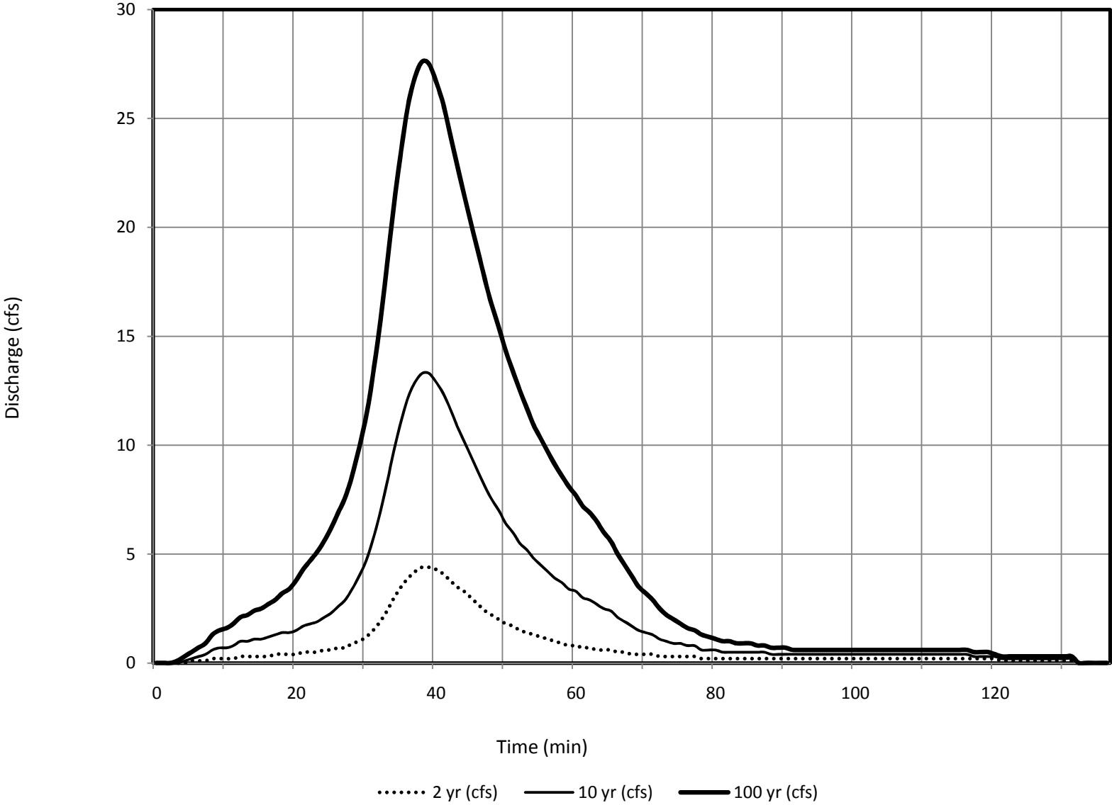
Subbasin 222 - DBDP Hydrologic Conditions
