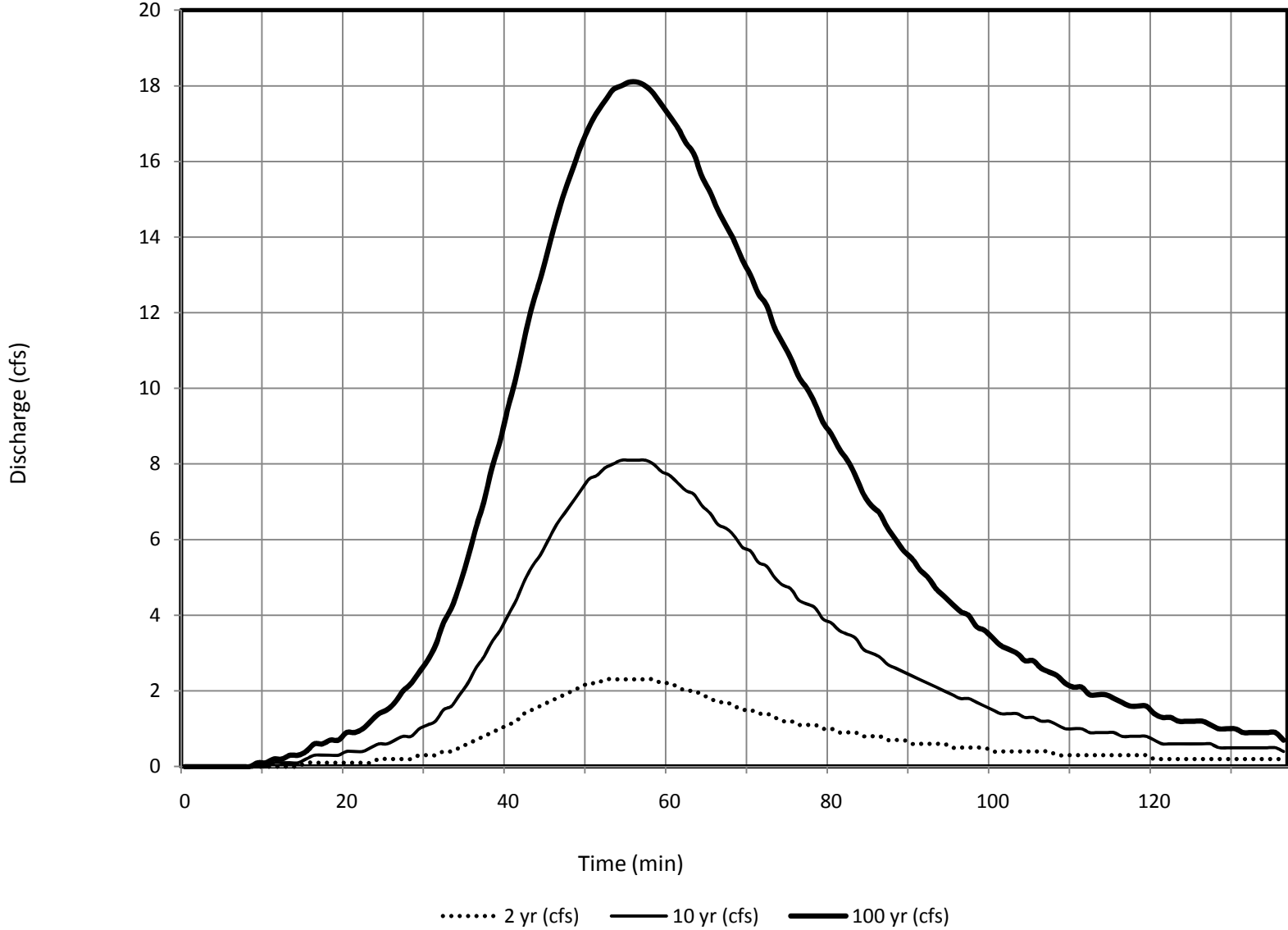
Subbasin 270 - DBDP Hydrologic Conditions
