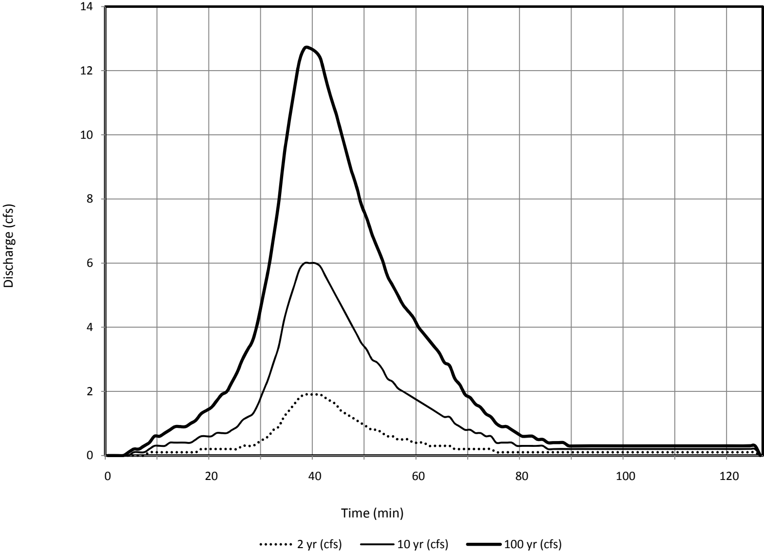
Subbasin 220 - DBDP Hydrologic Conditions
