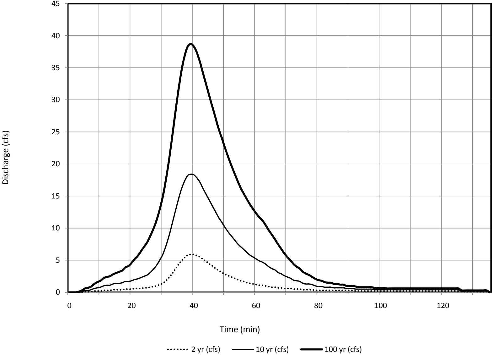
Subbasin 192 - DBDP Hydrologic Conditions
