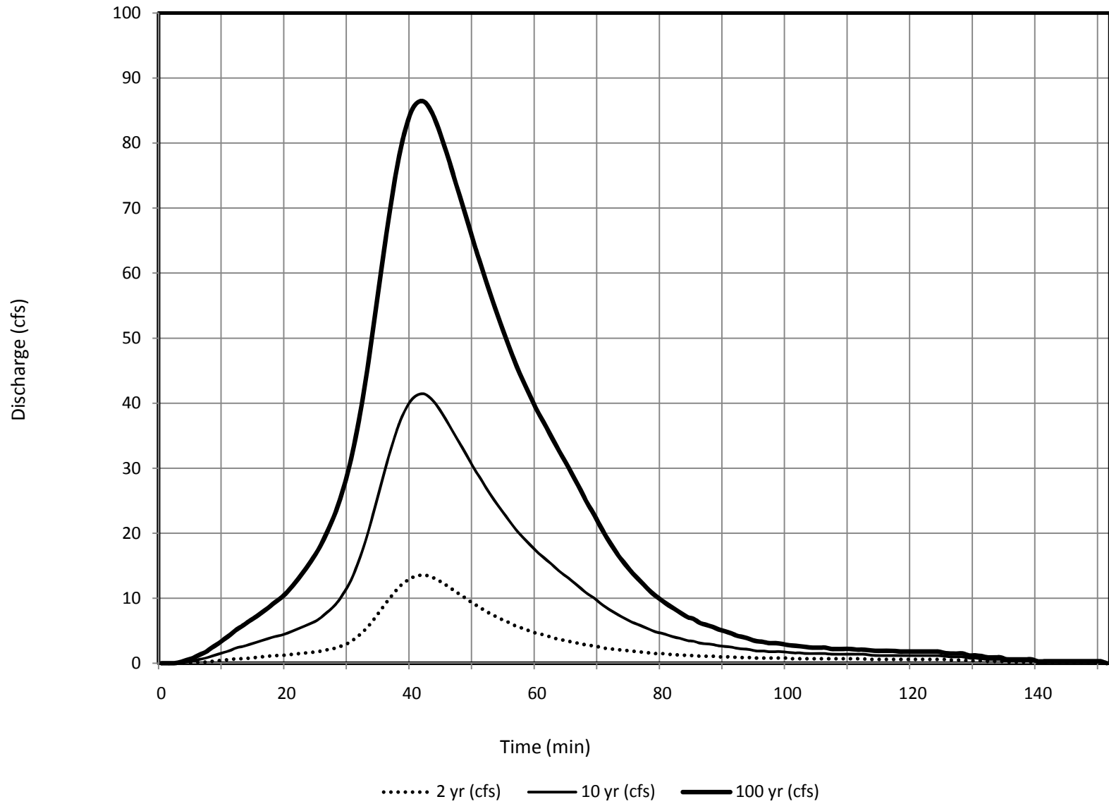
Subbasin 210 - DBDP Hydrologic Conditions
