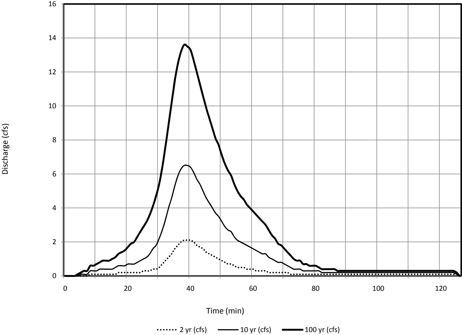
Subbasin 164 - DBDP Hydrologic Conditions
