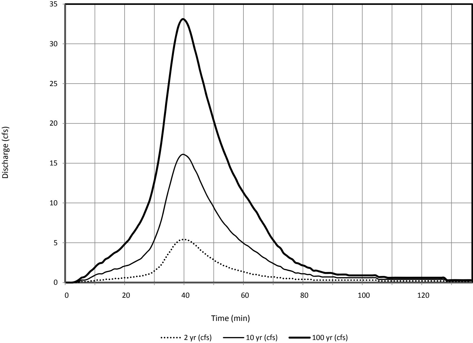
Subbasin 212 - DBDP Hydrologic Conditions
