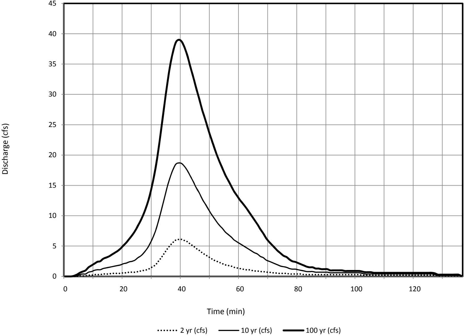
Subbasin 180 - DBDP Hydrologic Conditions
