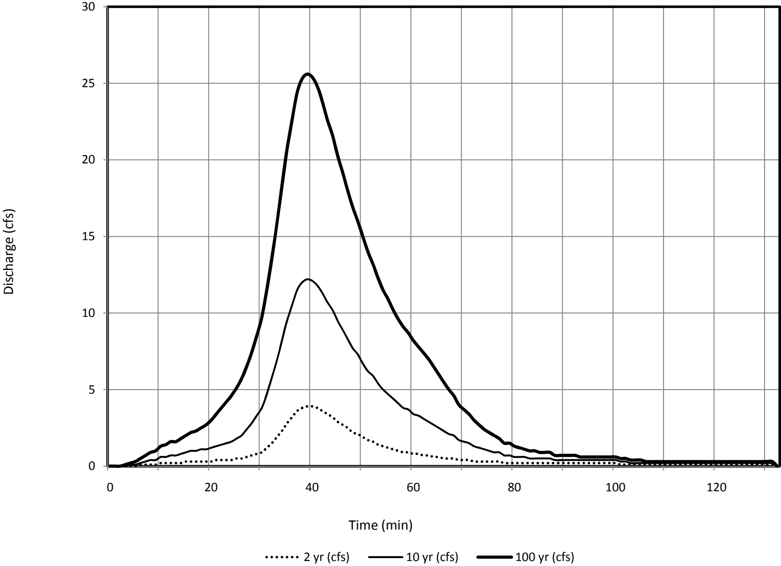
Subbasin 218 - DBDP Hydrologic Conditions
