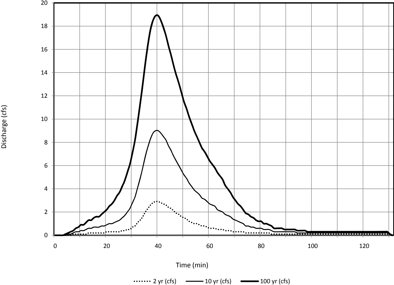
Subbasin 174 - DBDP Hydrologic Conditions
