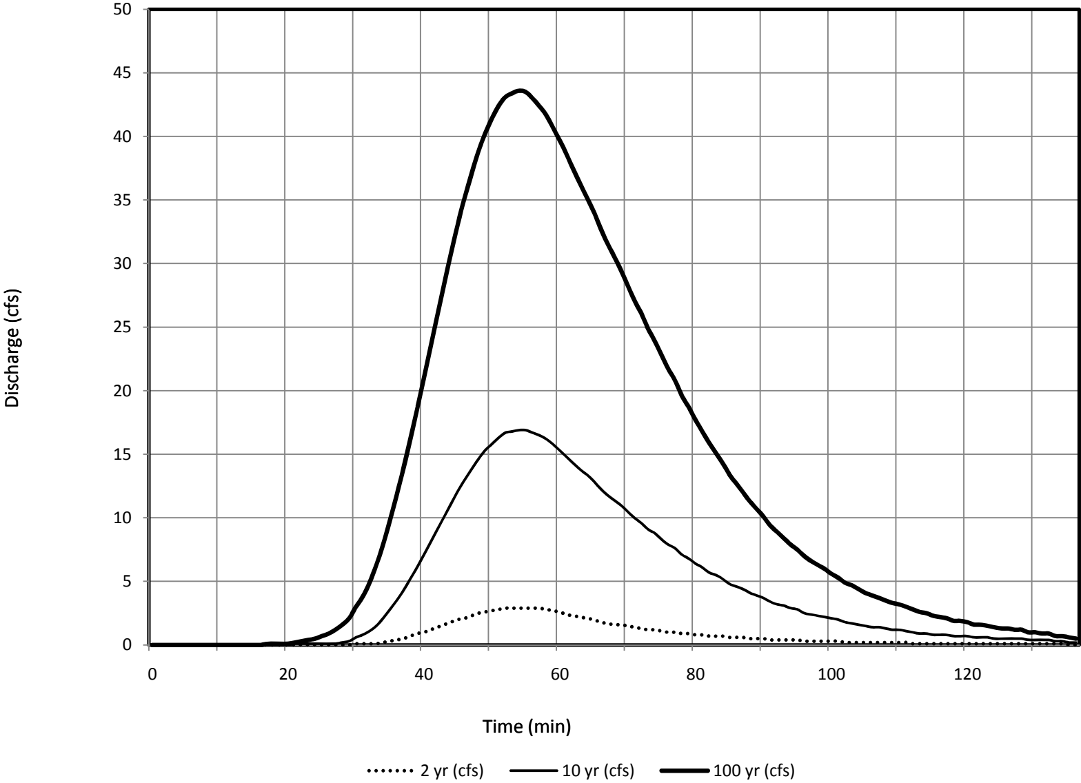
Subbasin 278 - DBDP Hydrologic Conditions
