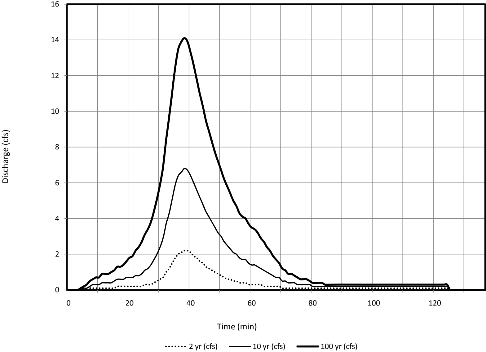
Subbasin 170 - DBDP Hydrologic Conditions
