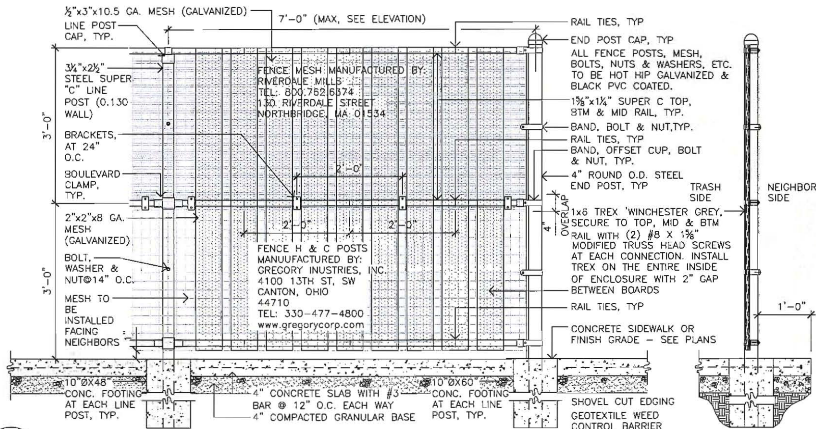
DETAIL: SECURITY 'NO-CLIMB' FENCE AT TRASH ENCLOSURE
