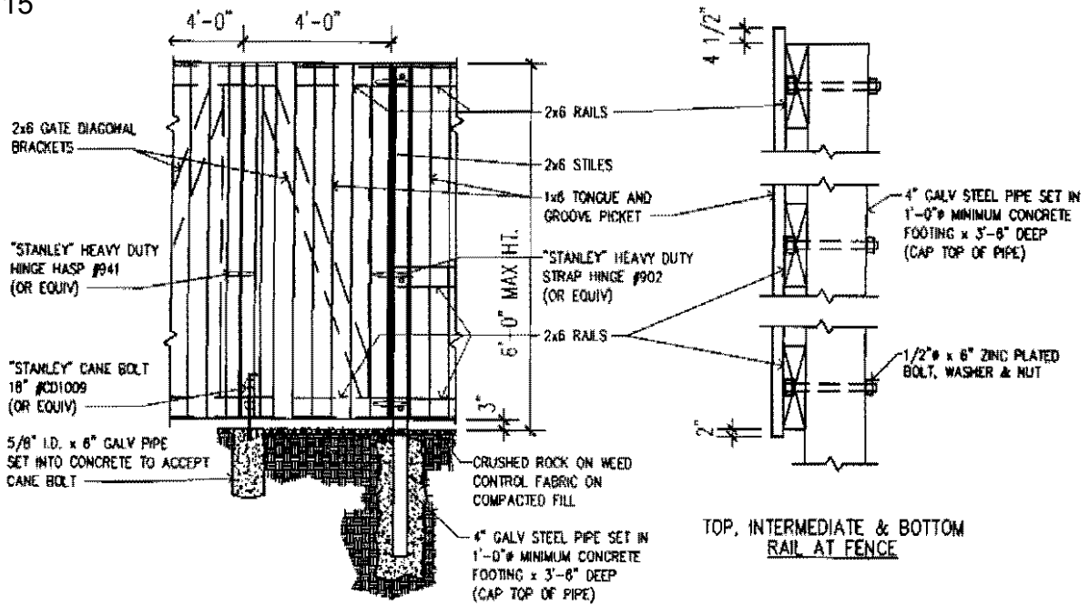
1 TYPICAL WOOD FENCE / GATE DETAIL SCALE: NOT TO SCALE
