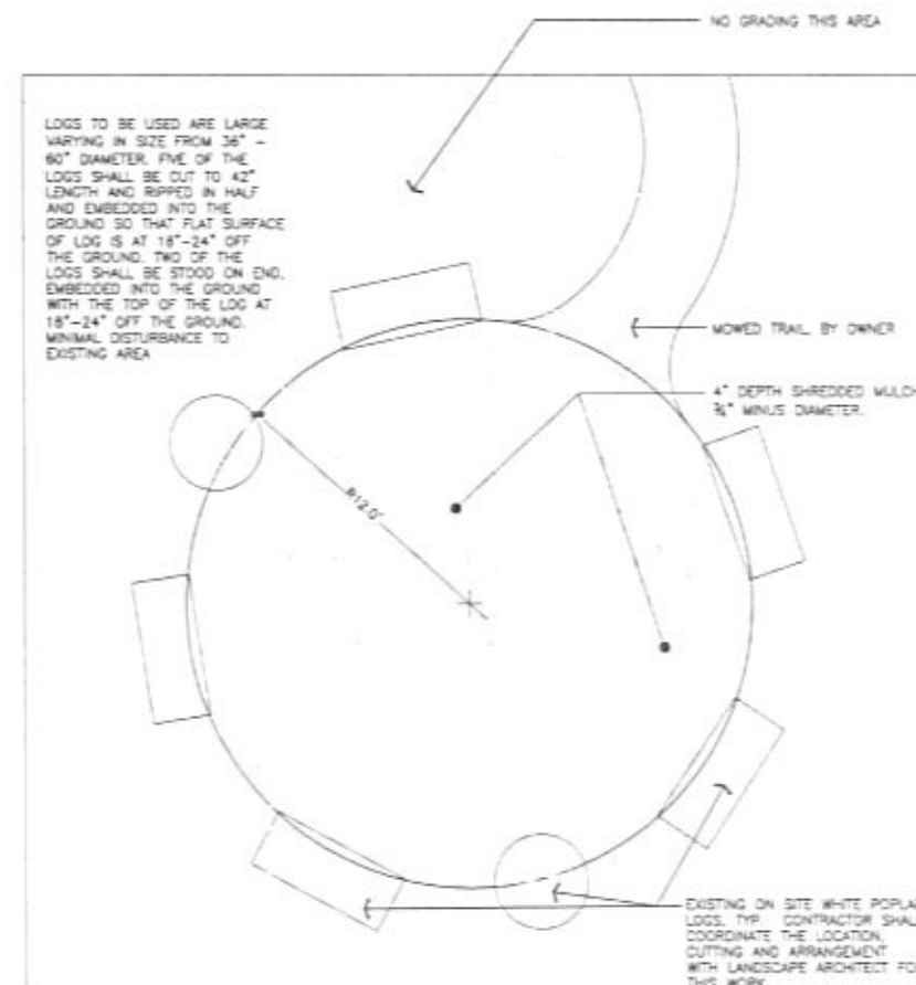
6 DETAIL: POPLAR GROVE COUNCIL RING L2.25 SCALE: 1/4" = 1'-0"
