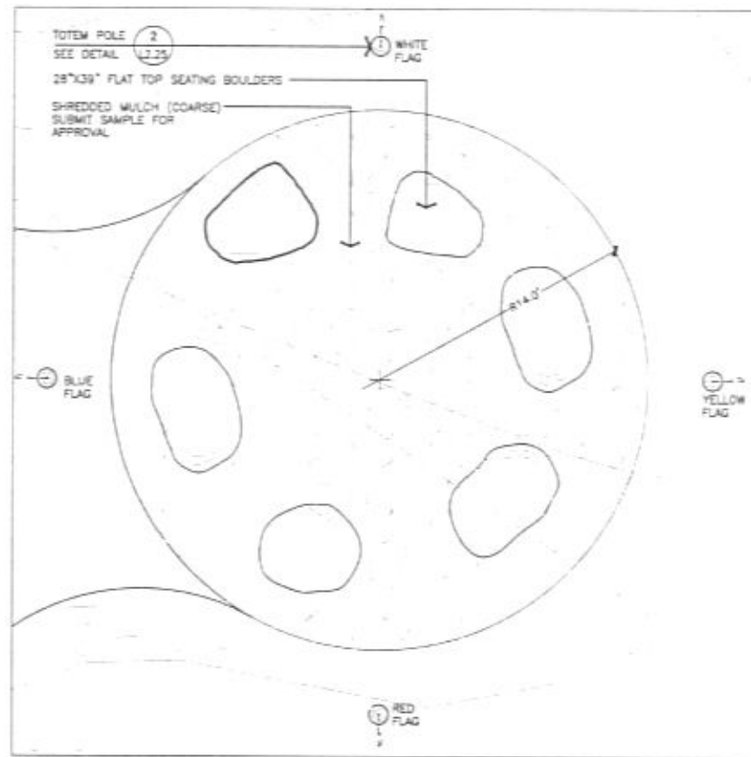
1 DETAIL: LIME CREEK COUNCIL RING L2.25 SCALE: 1/4" = 1'-0"
