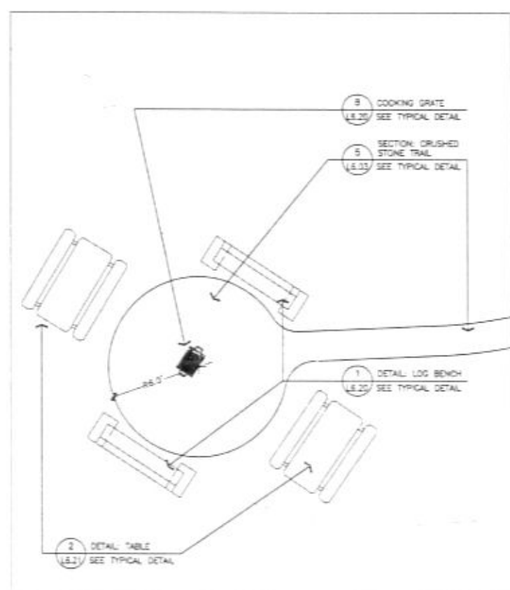
5 DETAIL: PICNIC / SEATING AREA L2.25 SCALE: 1/4" = 1'-0"
