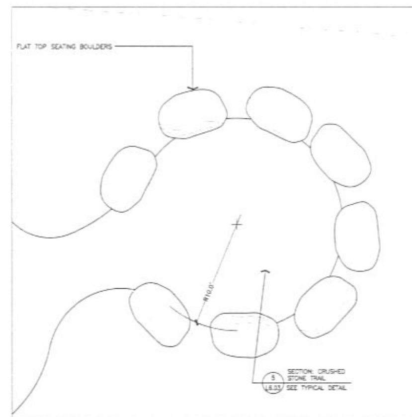
3 DETAIL: STONE HENGE COUNCIL RING L2.25 SCALE: 1/4" = 1'-0"
