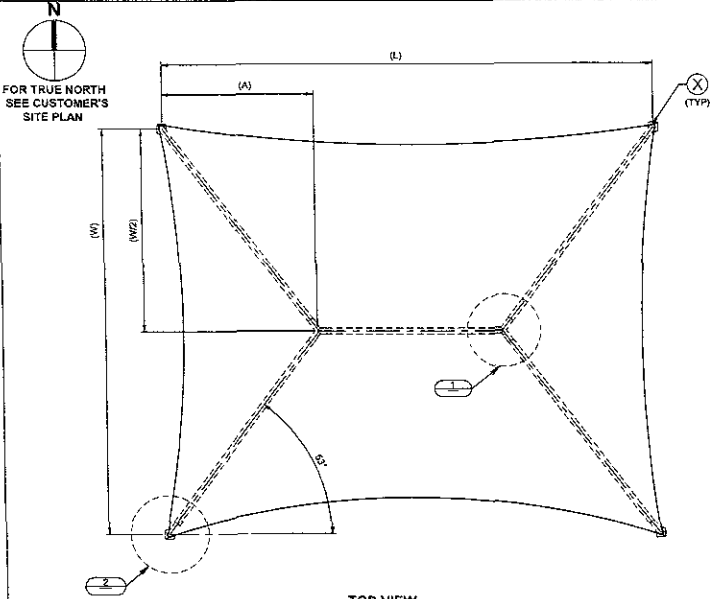
TOP VIEW (SCHEMATIC VIEW ONLY)
