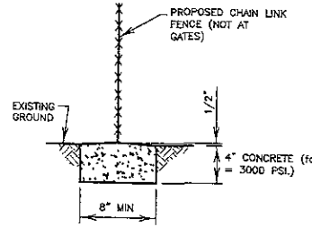
TYPICAL CONCRETE MOWING STRIP NOT TO SCALE
