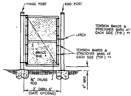
WALK GATE NOT TO SCALE
